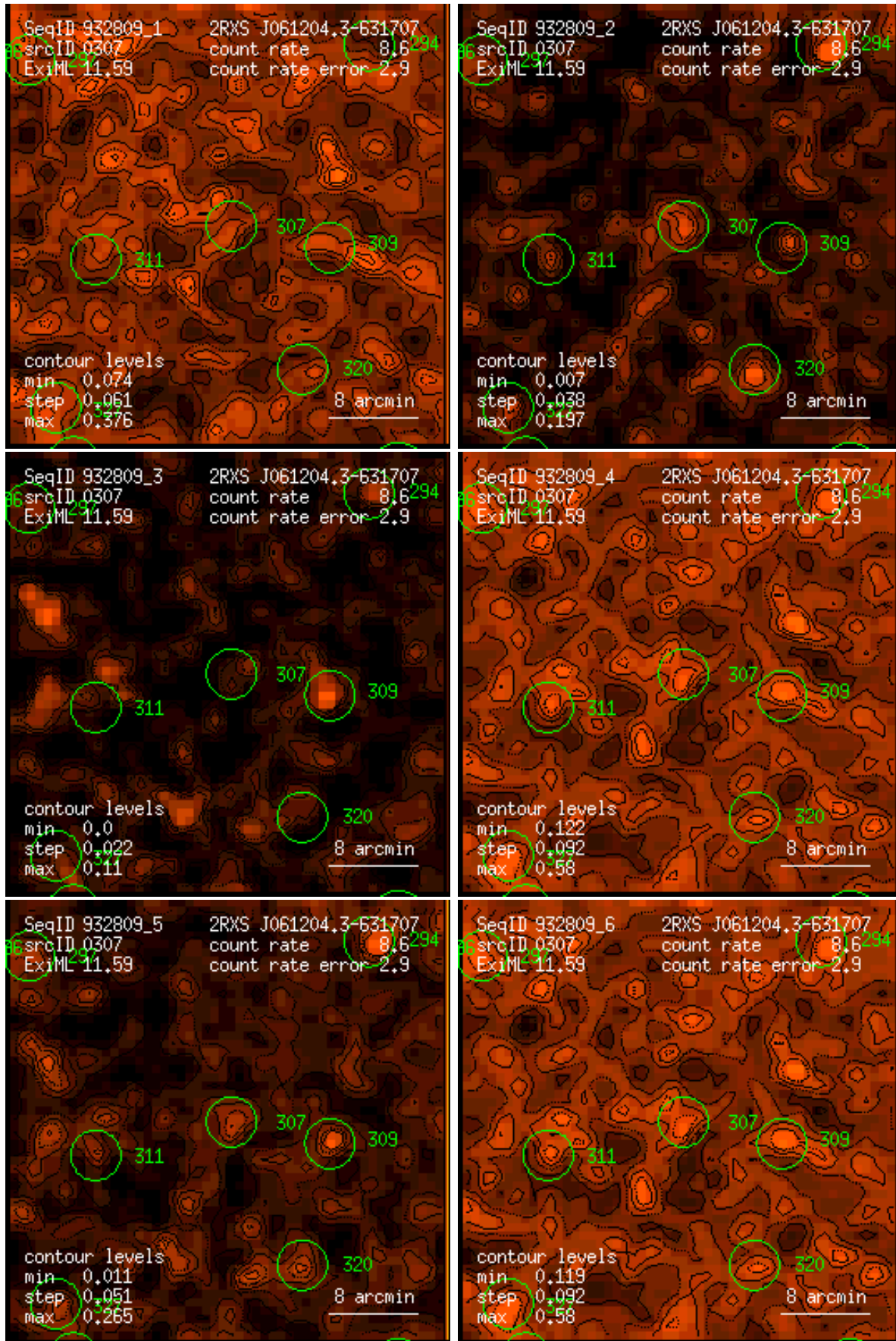
Figure 307: RASS 932809: detection 0307: band rate images, Gaussian filter: (1) PSPC channels 11 – 41, (2) 52 – 90, (3) 91 – 201, (4) 11 – 235, (5) 52 – 201, (6) 11 – 201. Broad band rates in counts/ks. Band rate contour levels in counts/ks/arcmin 2 .
