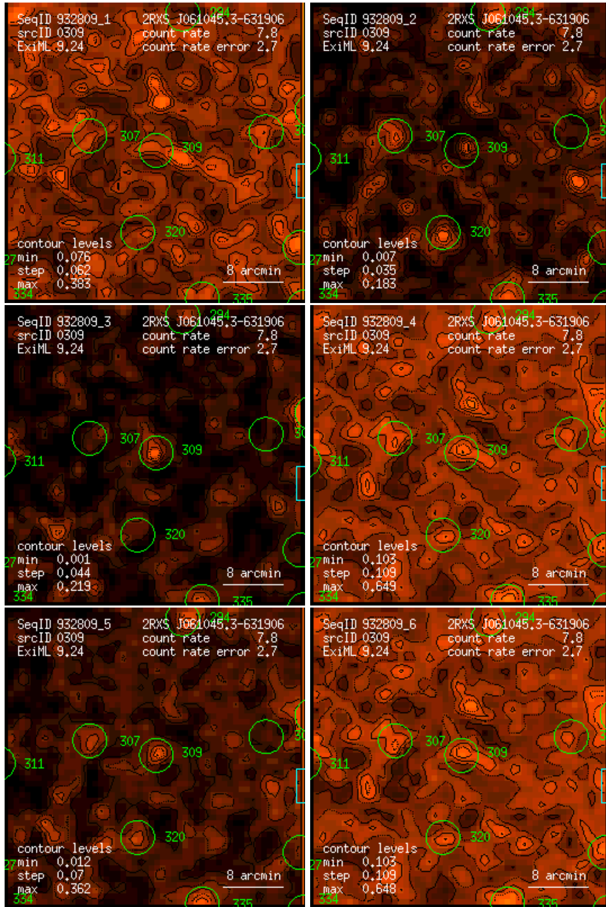
Figure 309: RASS 932809: detection 0309: band rate images, Gaussian filter: (1) PSPC channels 11 – 41, (2) 52 – 90, (3) 91 – 201, (4) 11 – 235, (5) 52 – 201, (6) 11 – 201. Broad band rates in counts/ks. Band rate contour levels in counts/ks/arcmin 2 .
