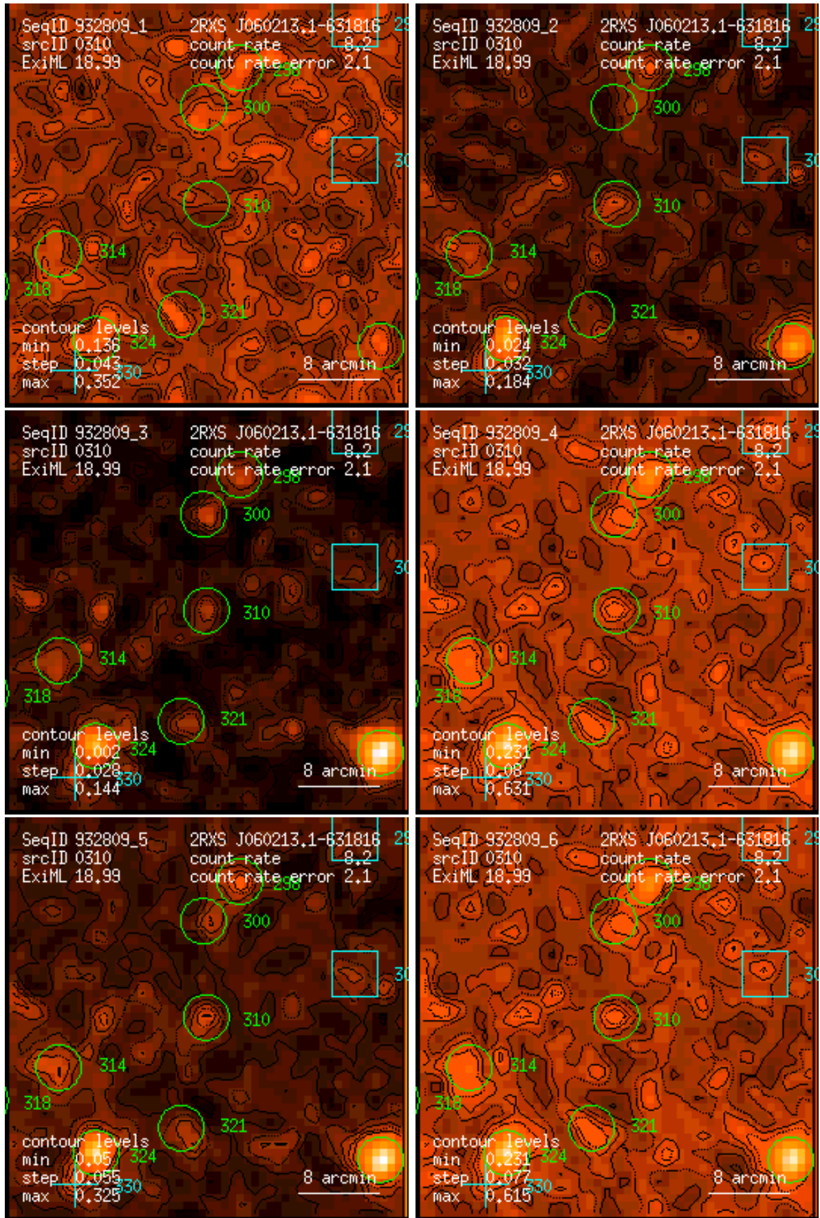
Figure 310: RASS 932809: detection 0310: band rate images, Gaussian filter: (1) PSPC channels 11 – 41, (2) 52 – 90, (3) 91 – 201, (4) 11 – 235, (5) 52 – 201, (6) 11 – 201. Broad band rates in counts/ks. Band rate contour levels in counts/ks/arcmin 2 .
