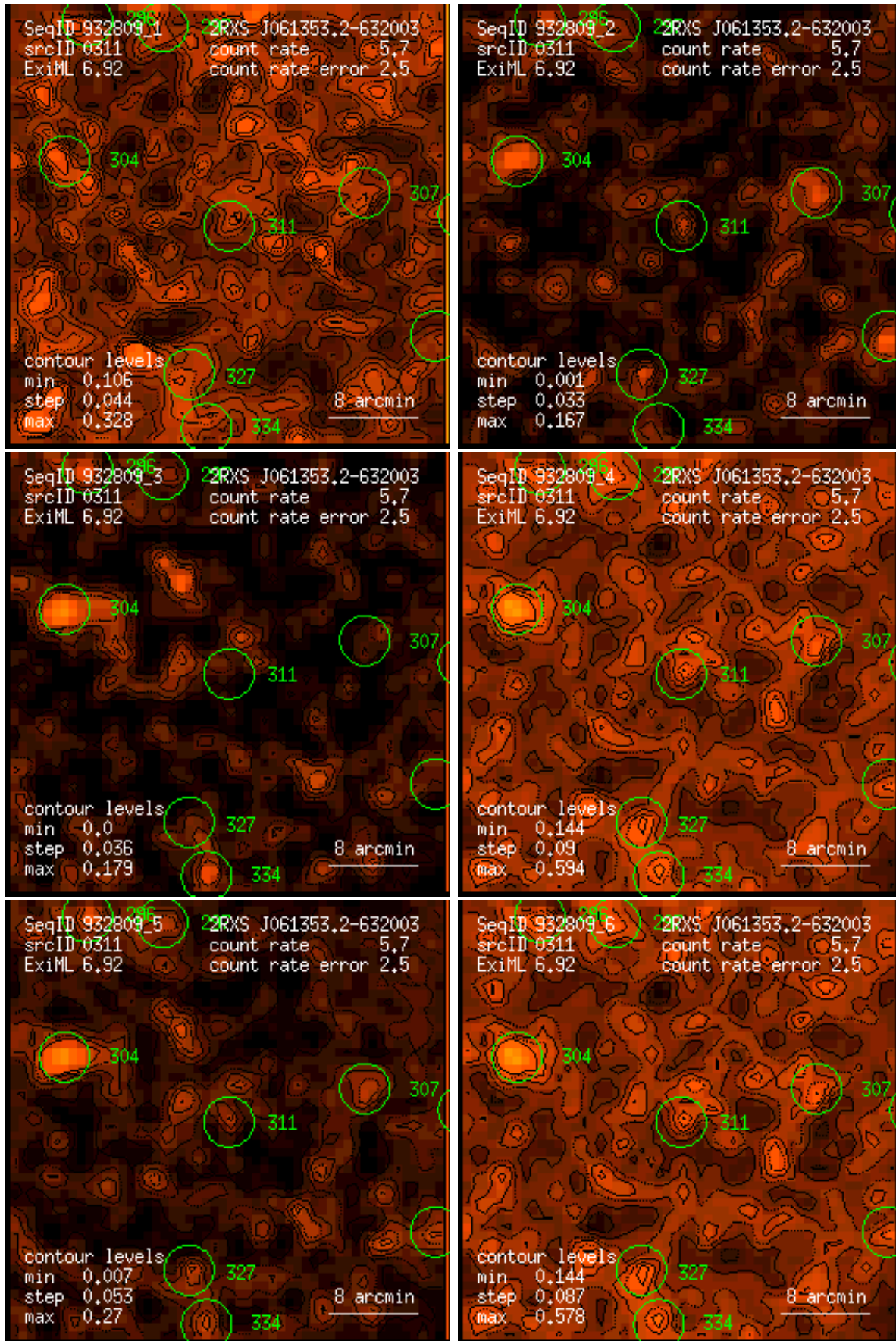
Figure 311: RASS 932809: detection 0311: band rate images, Gaussian filter: (1) PSPC channels 11 – 41, (2) 52 – 90, (3) 91 – 201, (4) 11 – 235, (5) 52 – 201, (6) 11 – 201. Broad band rates in counts/ks. Band rate contour levels in counts/ks/arcmin 2 .
