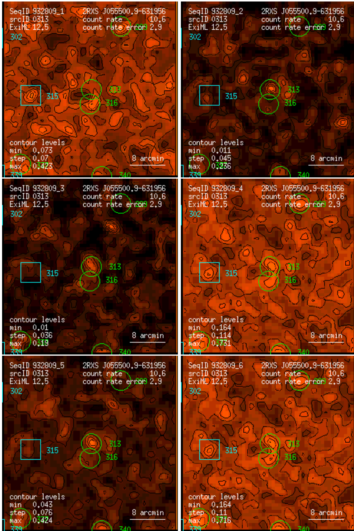
Figure 313: RASS 932809: detection 0313: band rate images, Gaussian filter: (1) PSPC channels 11 – 41, (2) 52 – 90, (3) 91 – 201, (4) 11 – 235, (5) 52 – 201, (6) 11 – 201. Broad band rates in counts/ks. Band rate contour levels in counts/ks/arcmin 2 .
