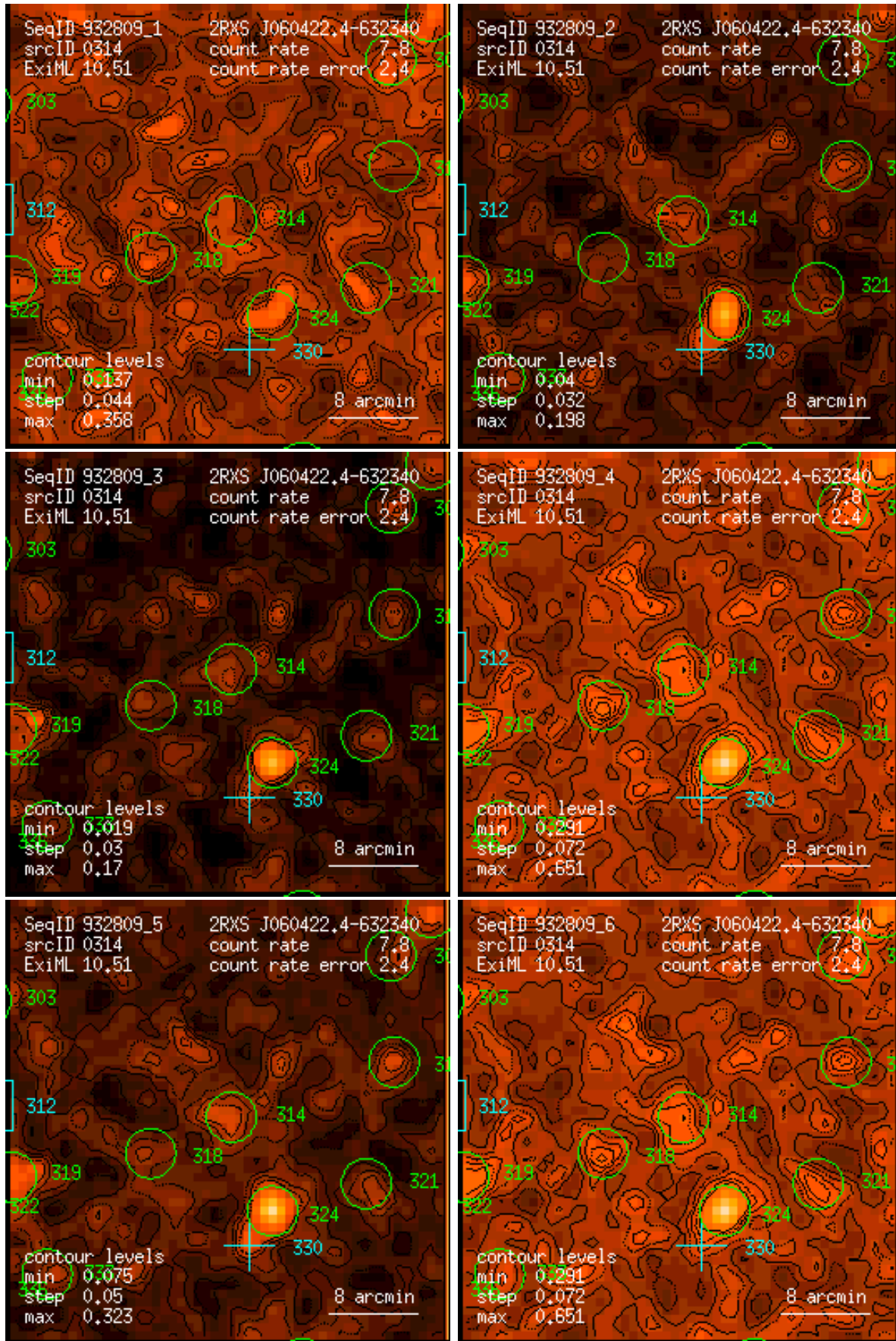
Figure 314: RASS 932809: detection 0314: band rate images, Gaussian filter: (1) PSPC channels 11 – 41, (2) 52 – 90, (3) 91 – 201, (4) 11 – 235, (5) 52 – 201, (6) 11 – 201. Broad band rates in counts/ks. Band rate contour levels in counts/ks/arcmin 2 .
