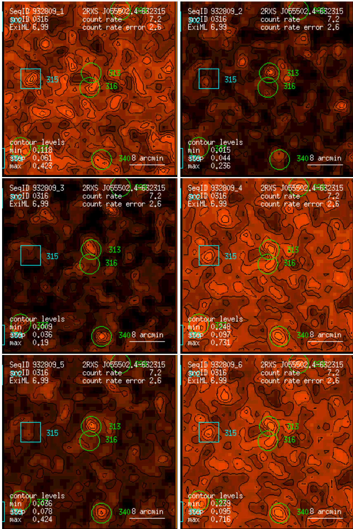
Figure 316: RASS 932809: detection 0316: band rate images, Gaussian filter: (1) PSPC channels 11 – 41, (2) 52 – 90, (3) 91 – 201, (4) 11 – 235, (5) 52 – 201, (6) 11 – 201. Broad band rates in counts/ks. Band rate contour levels in counts/ks/arcmin 2 .
