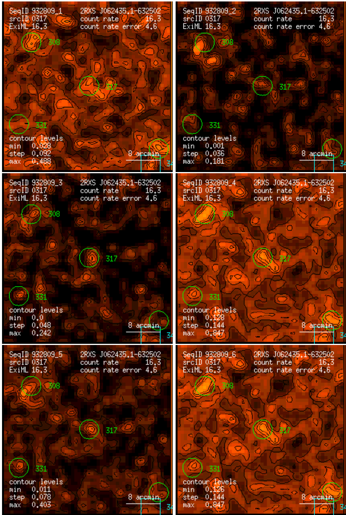
Figure 317: RASS 932809: detection 0317: band rate images, Gaussian filter: (1) PSPC channels 11 – 41, (2) 52 – 90, (3) 91 – 201, (4) 11 – 235, (5) 52 – 201, (6) 11 – 201. Broad band rates in counts/ks. Band rate contour levels in counts/ks/arcmin 2 .
