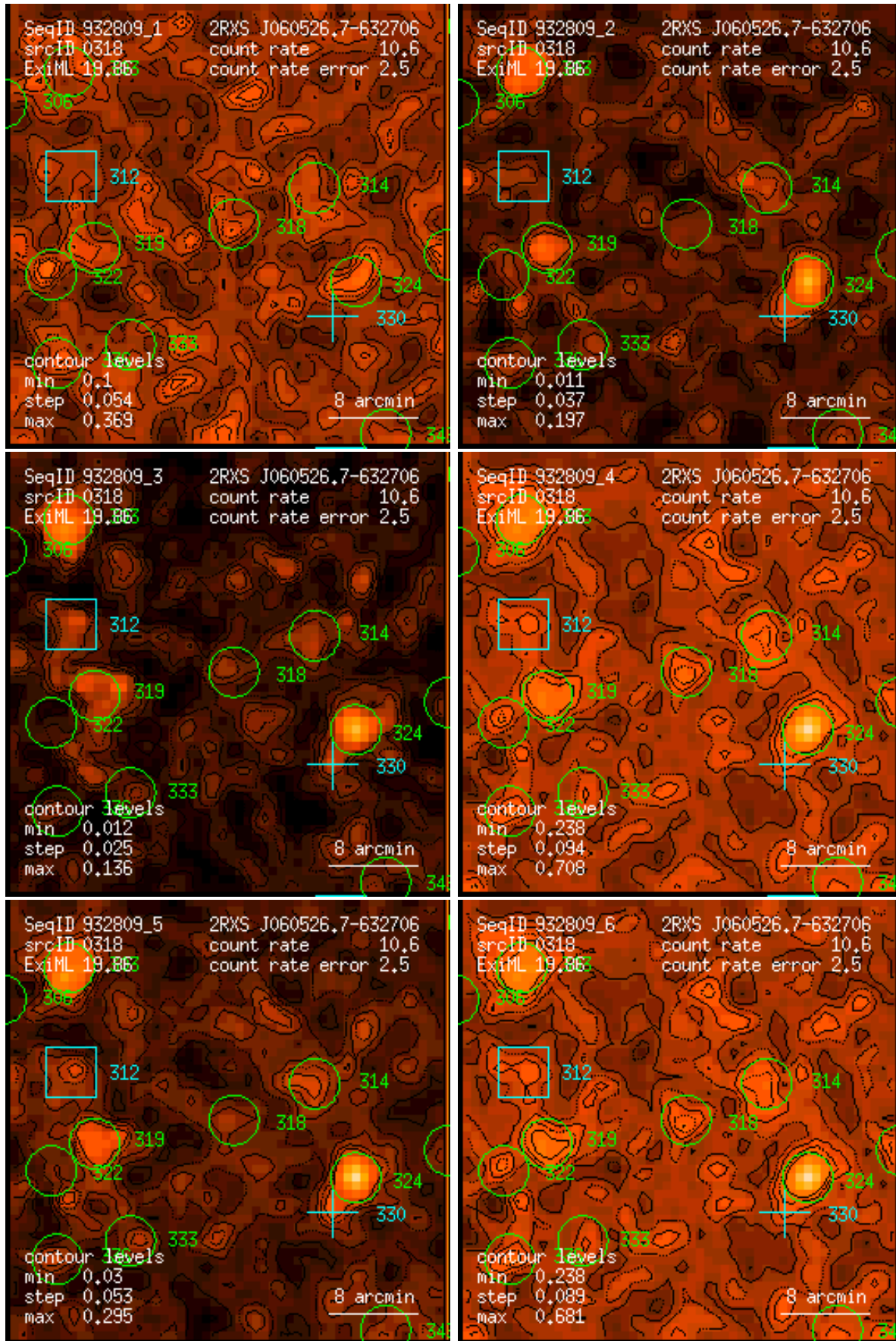
Figure 318: RASS 932809: detection 0318: band rate images, Gaussian filter: (1) PSPC channels 11 – 41, (2) 52 – 90, (3) 91 – 201, (4) 11 – 235, (5) 52 – 201, (6) 11 – 201. Broad band rates in counts/ks. Band rate contour levels in counts/ks/arcmin 2 .
