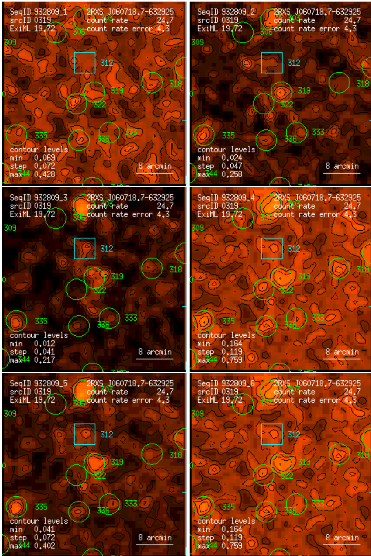
Figure 319: RASS 932809: detection 0319: band rate images, Gaussian filter: (1) PSPC channels 11 – 41, (2) 52 – 90, (3) 91 – 201, (4) 11 – 235, (5) 52 – 201, (6) 11 – 201. Broad band rates in counts/ks. Band rate contour levels in counts/ks/arcmin 2 .
