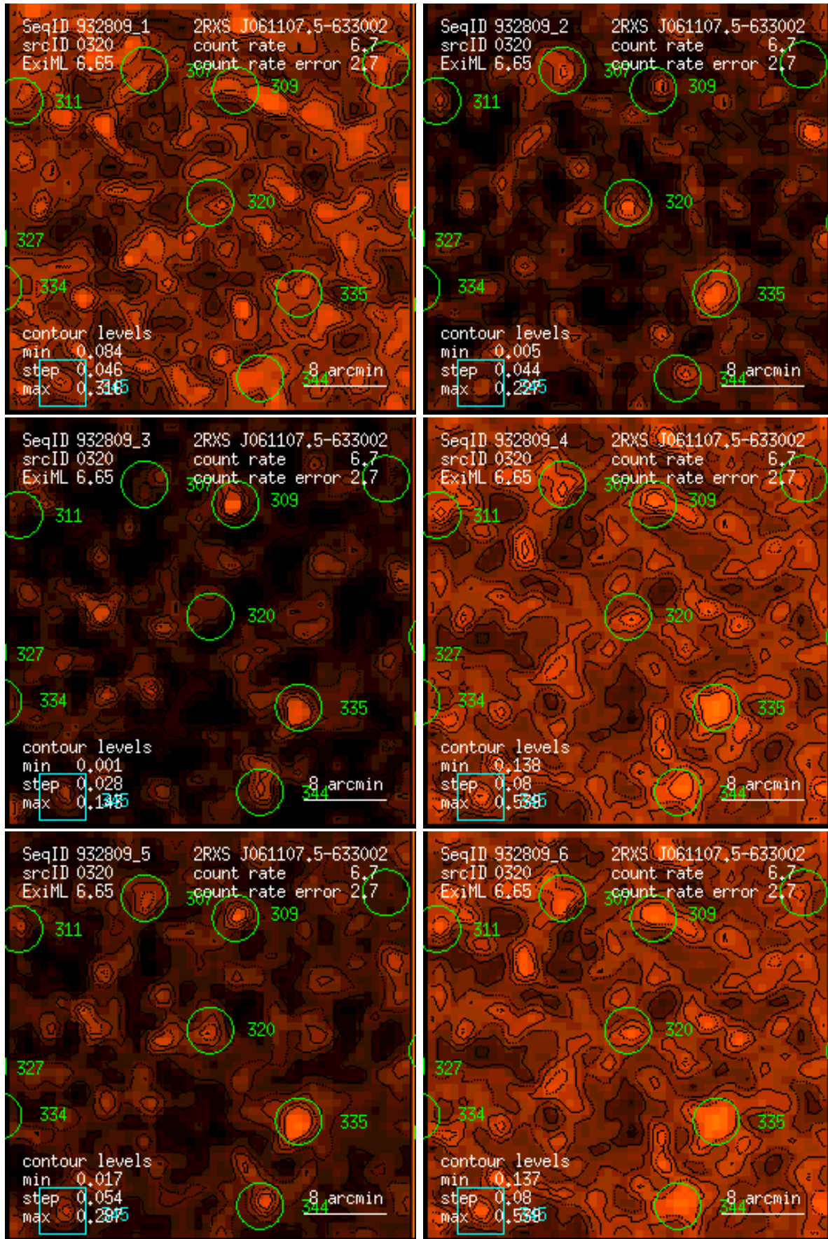
Figure 320: RASS 932809: detection 0320: band rate images, Gaussian filter: (1) PSPC channels 11 – 41, (2) 52 – 90, (3) 91 – 201, (4) 11 – 235, (5) 52 – 201, (6) 11 – 201. Broad band rates in counts/ks. Band rate contour levels in counts/ks/arcmin 2 .
