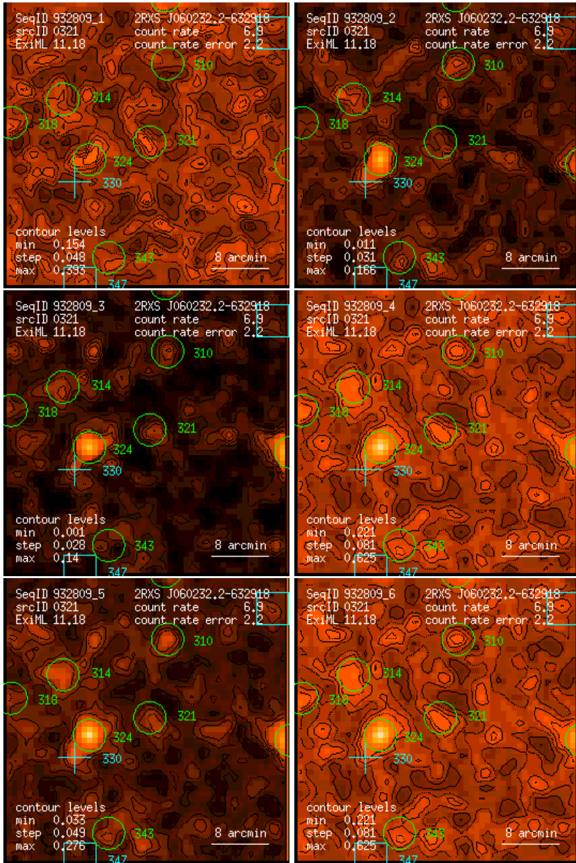
Figure 321: RASS 932809: detection 0321: band rate images, Gaussian filter: (1) PSPC channels 11 – 41, (2) 52 – 90, (3) 91 – 201, (4) 11 – 235, (5) 52 – 201, (6) 11 – 201. Broad band rates in counts/ks. Band rate contour levels in counts/ks/arcmin 2 .
