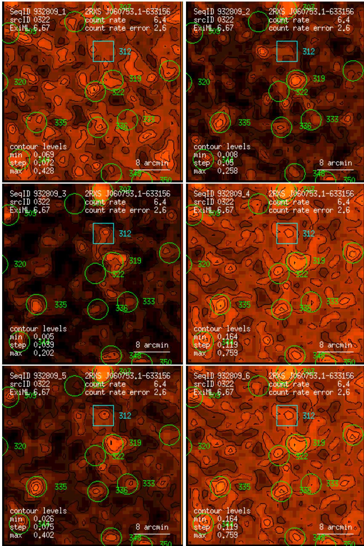
Figure 322: RASS 932809: detection 0322: band rate images, Gaussian filter: (1) PSPC channels 11 – 41, (2) 52 – 90, (3) 91 – 201, (4) 11 – 235, (5) 52 – 201, (6) 11 – 201. Broad band rates in counts/ks. Band rate contour levels in counts/ks/arcmin 2 .
