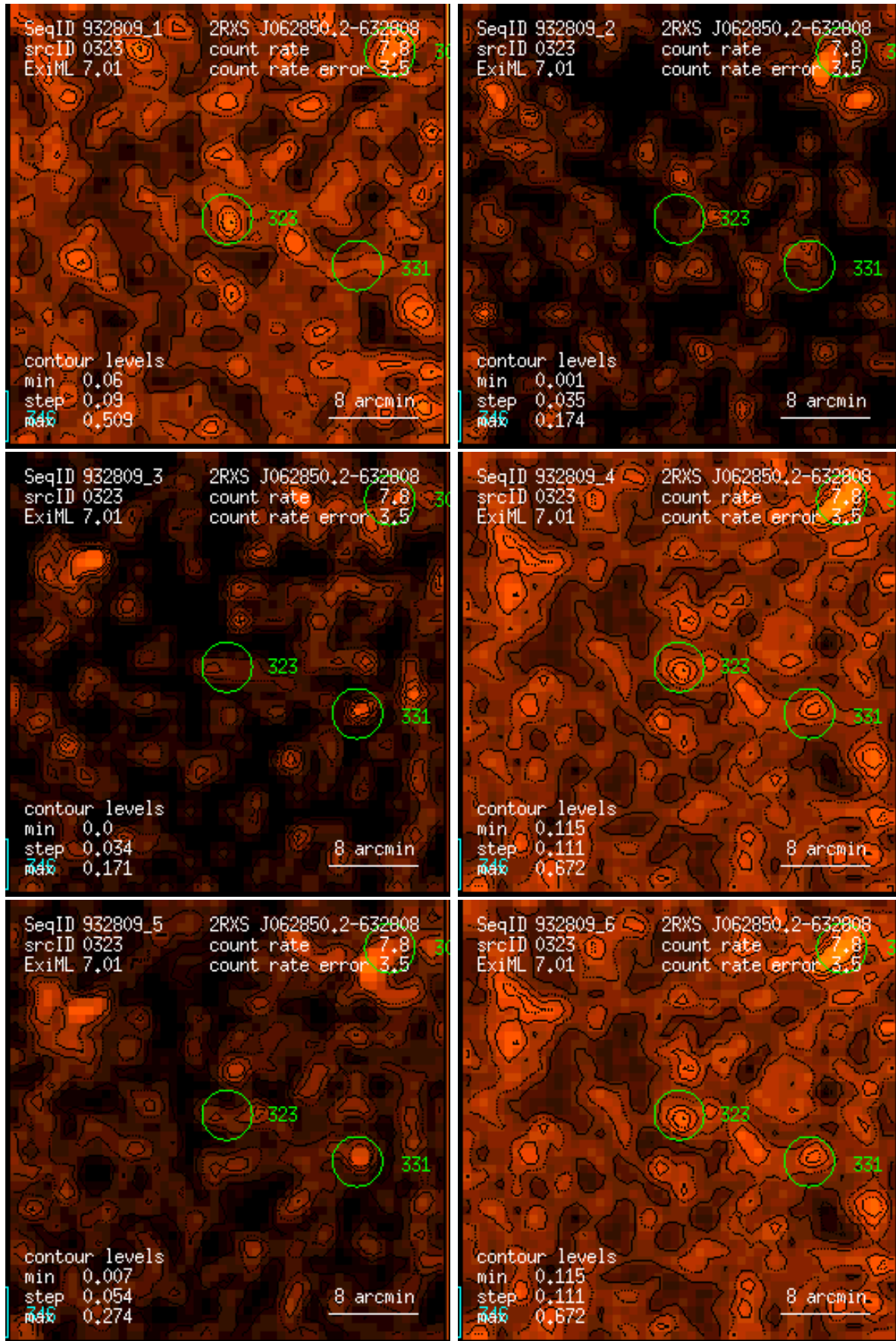
Figure 323: RASS 932809: detection 0323: band rate images, Gaussian filter: (1) PSPC channels 11 – 41, (2) 52 – 90, (3) 91 – 201, (4) 11 – 235, (5) 52 – 201, (6) 11 – 201. Broad band rates in counts/ks. Band rate contour levels in counts/ks/arcmin 2 .
