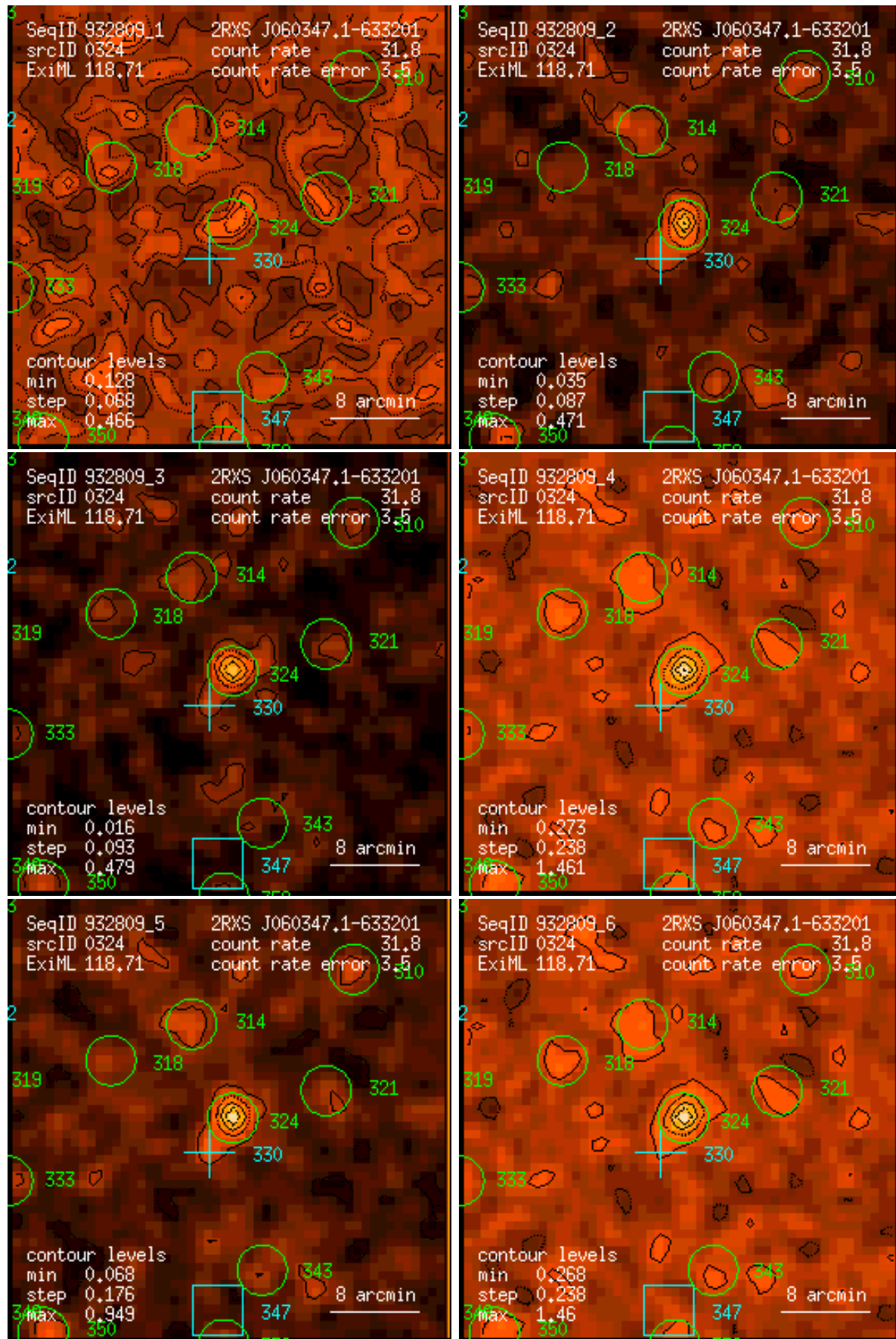
Figure 324: RASS 932809: detection 0324: band rate images, Gaussian filter: (1) PSPC channels 11 – 41, (2) 52 – 90, (3) 91 – 201, (4) 11 – 235, (5) 52 – 201, (6) 11 – 201. Broad band rates in counts/ks. Band rate contour levels in counts/ks/arcmin 2 .
