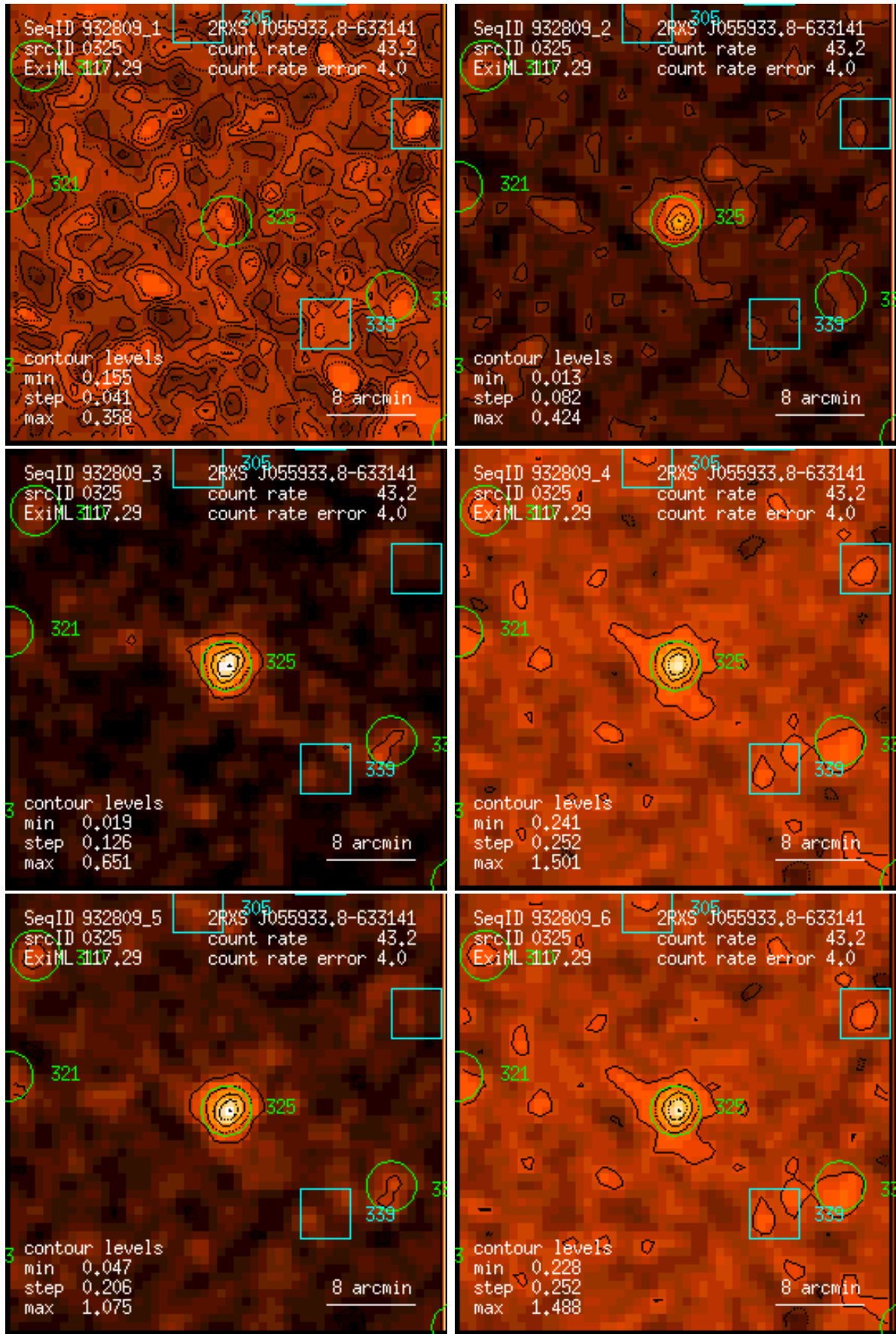
Figure 325: RASS 932809: detection 0325: band rate images, Gaussian filter: (1) PSPC channels 11 – 41, (2) 52 – 90, (3) 91 – 201, (4) 11 – 235, (5) 52 – 201, (6) 11 – 201. Broad band rates in counts/ks. Band rate contour levels in counts/ks/arcmin 2 .
