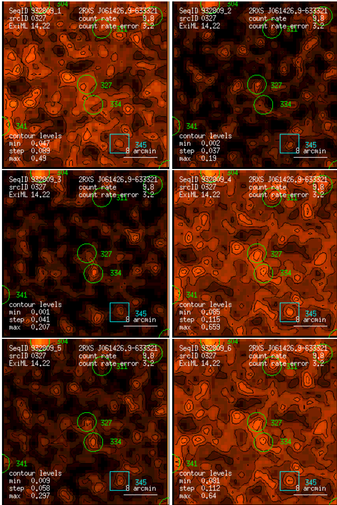
Figure 327: RASS 932809: detection 0327: band rate images, Gaussian filter: (1) PSPC channels 11 – 41, (2) 52 – 90, (3) 91 – 201, (4) 11 – 235, (5) 52 – 201, (6) 11 – 201. Broad band rates in counts/ks. Band rate contour levels in counts/ks/arcmin 2 .
