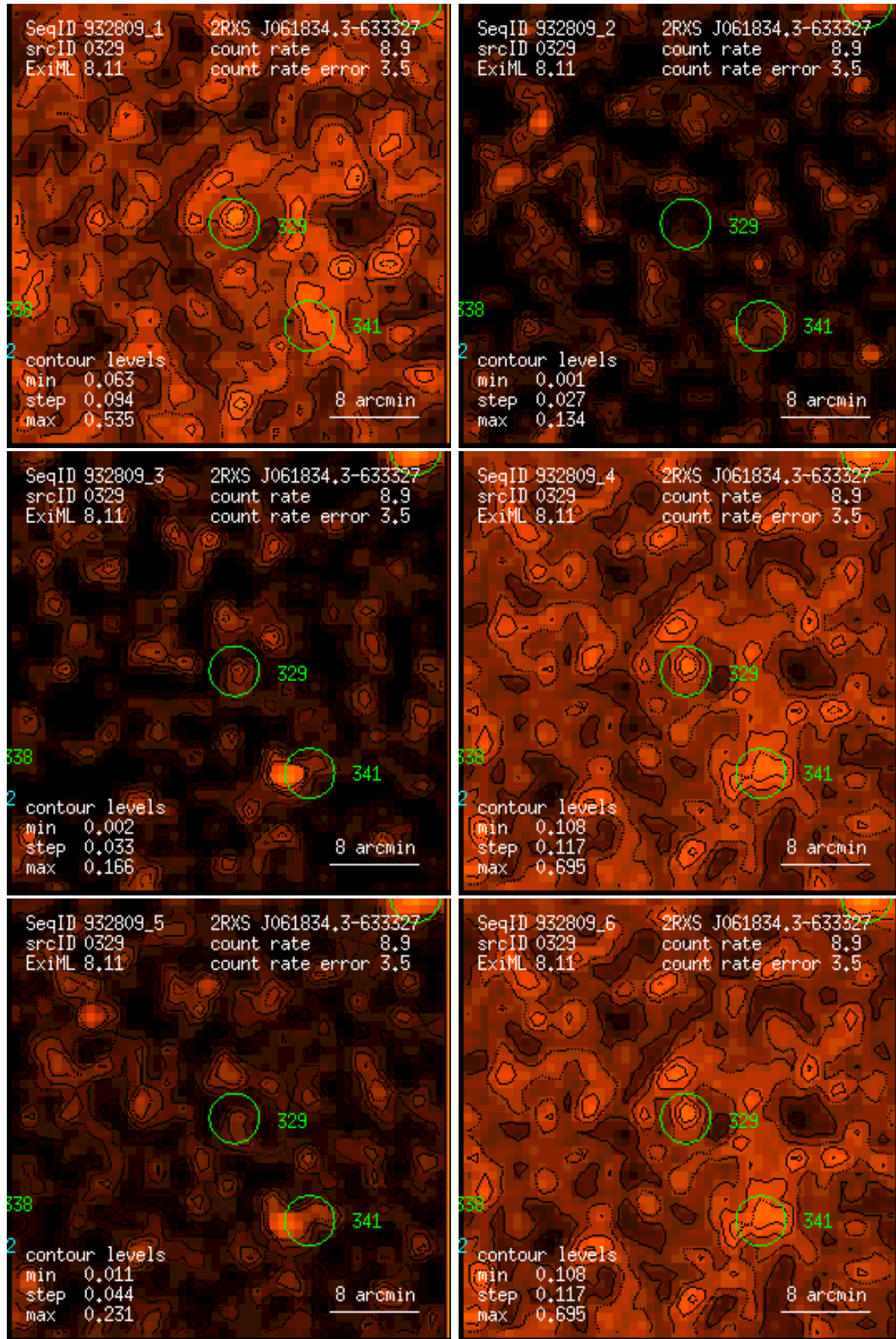
Figure 329: RASS 932809: detection 0329: band rate images, Gaussian filter: (1) PSPC channels 11 – 41, (2) 52 – 90, (3) 91 – 201, (4) 11 – 235, (5) 52 – 201, (6) 11 – 201. Broad band rates in counts/ks. Band rate contour levels in counts/ks/arcmin 2 .
