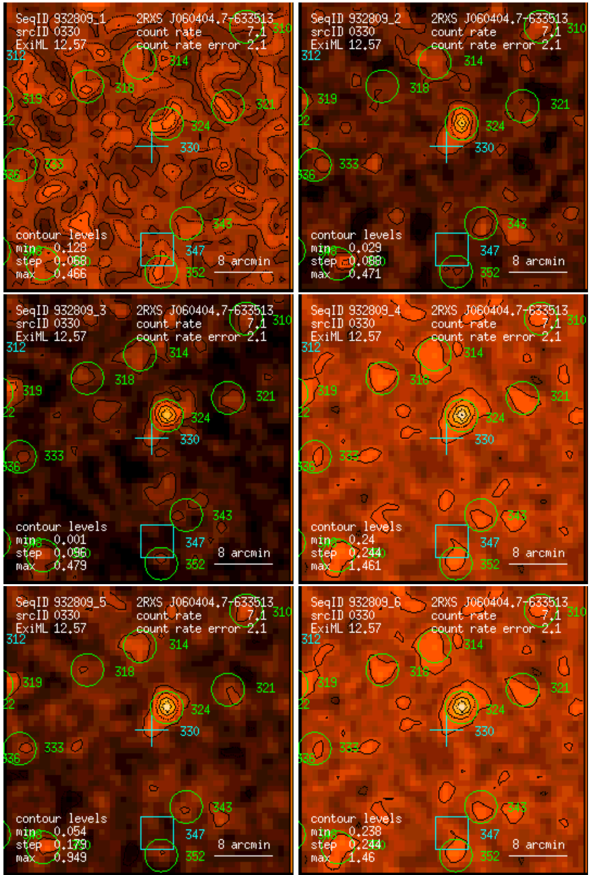
Figure 330: RASS 932809: detection 0330: band rate images, Gaussian filter: (1) PSPC channels 11 – 41, (2) 52 – 90, (3) 91 – 201, (4) 11 – 235, (5) 52 – 201, (6) 11 – 201. Broad band rates in counts/ks. Band rate contour levels in counts/ks/arcmin 2 .
