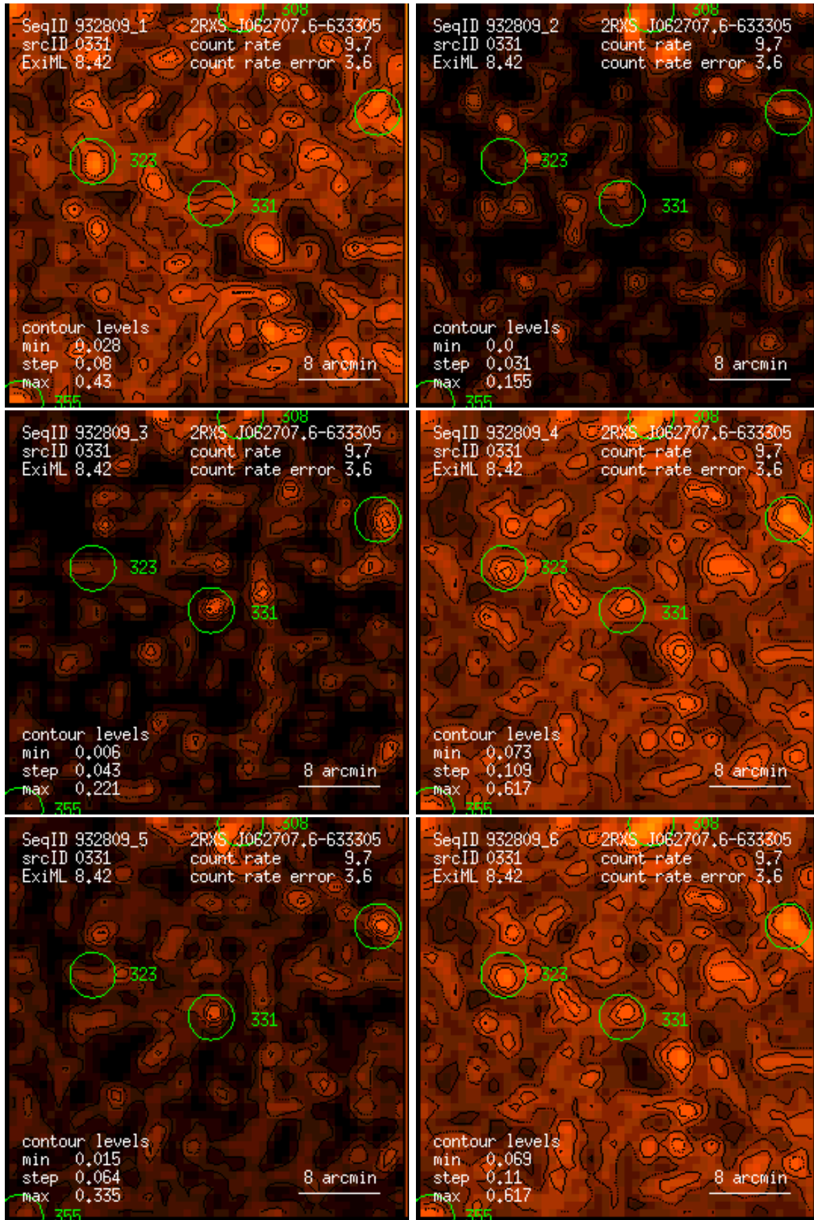
Figure 331: RASS 932809: detection 0331: band rate images, Gaussian filter: (1) PSPC channels 11 – 41, (2) 52 – 90, (3) 91 – 201, (4) 11 – 235, (5) 52 – 201, (6) 11 – 201. Broad band rates in counts/ks. Band rate contour levels in counts/ks/arcmin 2 .
