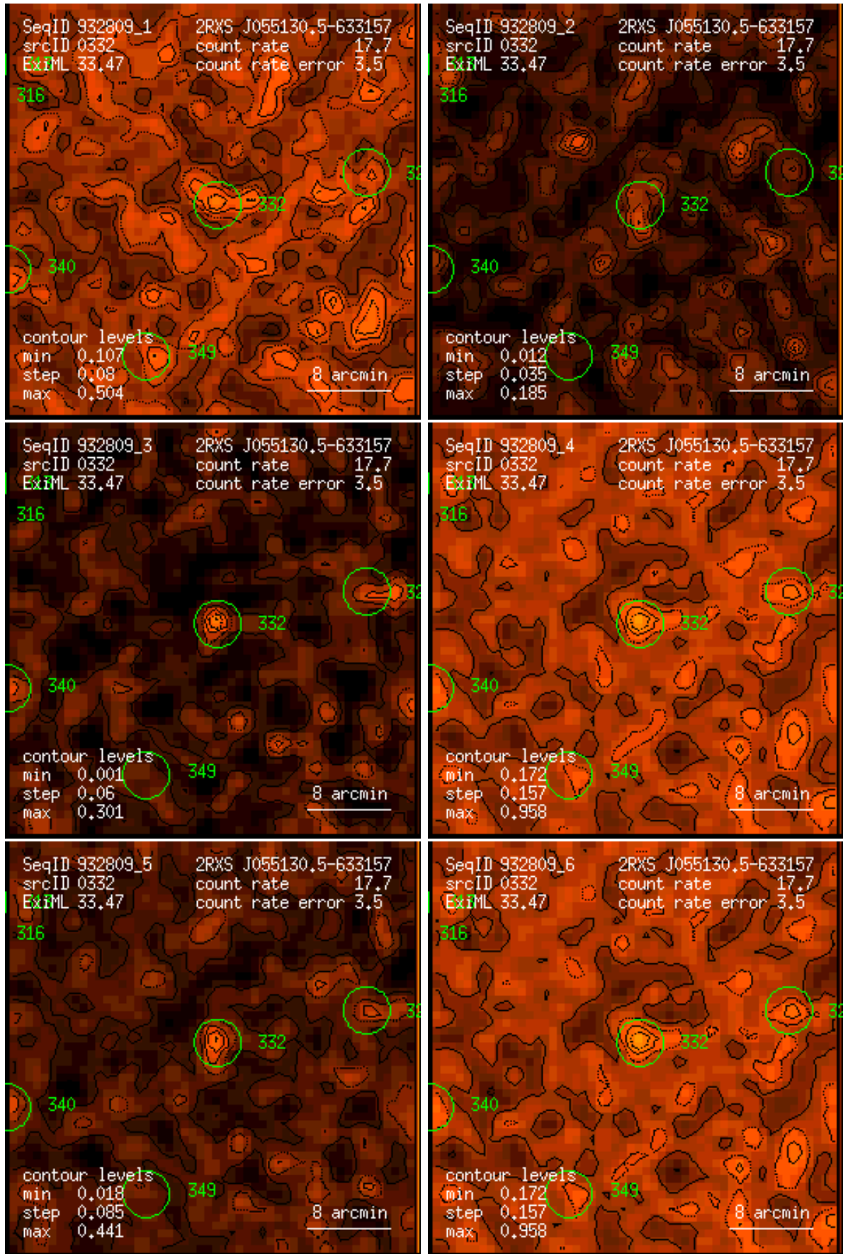
Figure 332: RASS 932809: detection 0332: band rate images, Gaussian filter: (1) PSPC channels 11 – 41, (2) 52 – 90, (3) 91 – 201, (4) 11 – 235, (5) 52 – 201, (6) 11 – 201. Broad band rates in counts/ks. Band rate contour levels in counts/ks/arcmin 2 .
