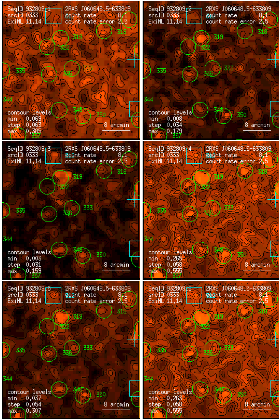
Figure 333: RASS 932809: detection 0333: band rate images, Gaussian filter: (1) PSPC channels 11 – 41, (2) 52 – 90, (3) 91 – 201, (4) 11 – 235, (5) 52 – 201, (6) 11 – 201. Broad band rates in counts/ks. Band rate contour levels in counts/ks/arcmin 2 .
