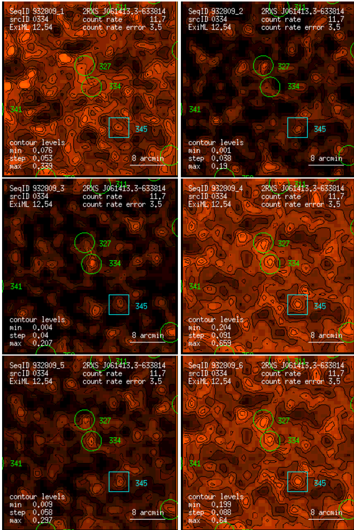
Figure 334: RASS 932809: detection 0334: band rate images, Gaussian filter: (1) PSPC channels 11 – 41, (2) 52 – 90, (3) 91 – 201, (4) 11 – 235, (5) 52 – 201, (6) 11 – 201. Broad band rates in counts/ks. Band rate contour levels in counts/ks/arcmin 2 .
