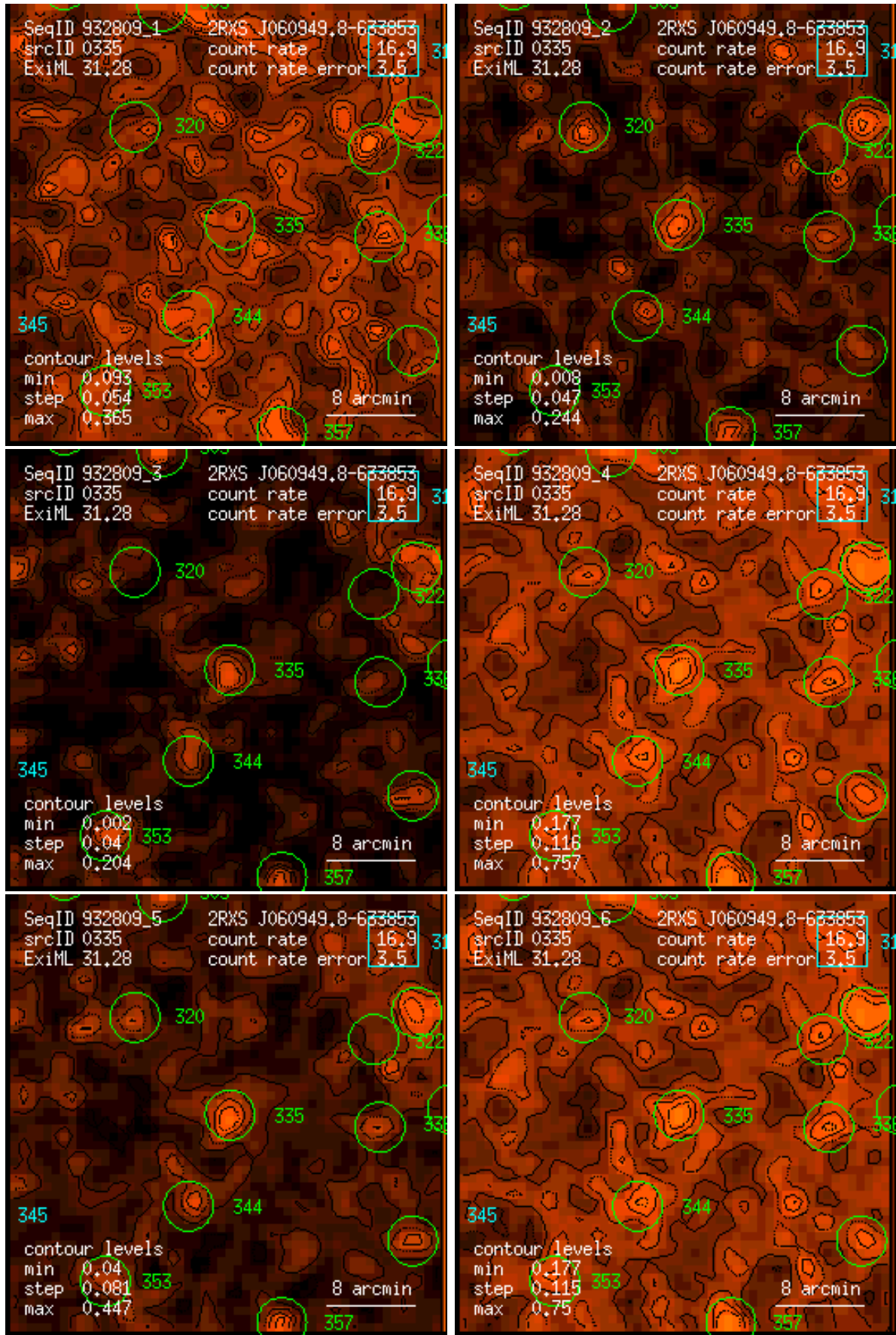
Figure 335: RASS 932809: detection 0335: band rate images, Gaussian filter: (1) PSPC channels 11 – 41, (2) 52 – 90, (3) 91 – 201, (4) 11 – 235, (5) 52 – 201, (6) 11 – 201. Broad band rates in counts/ks. Band rate contour levels in counts/ks/arcmin 2 .
