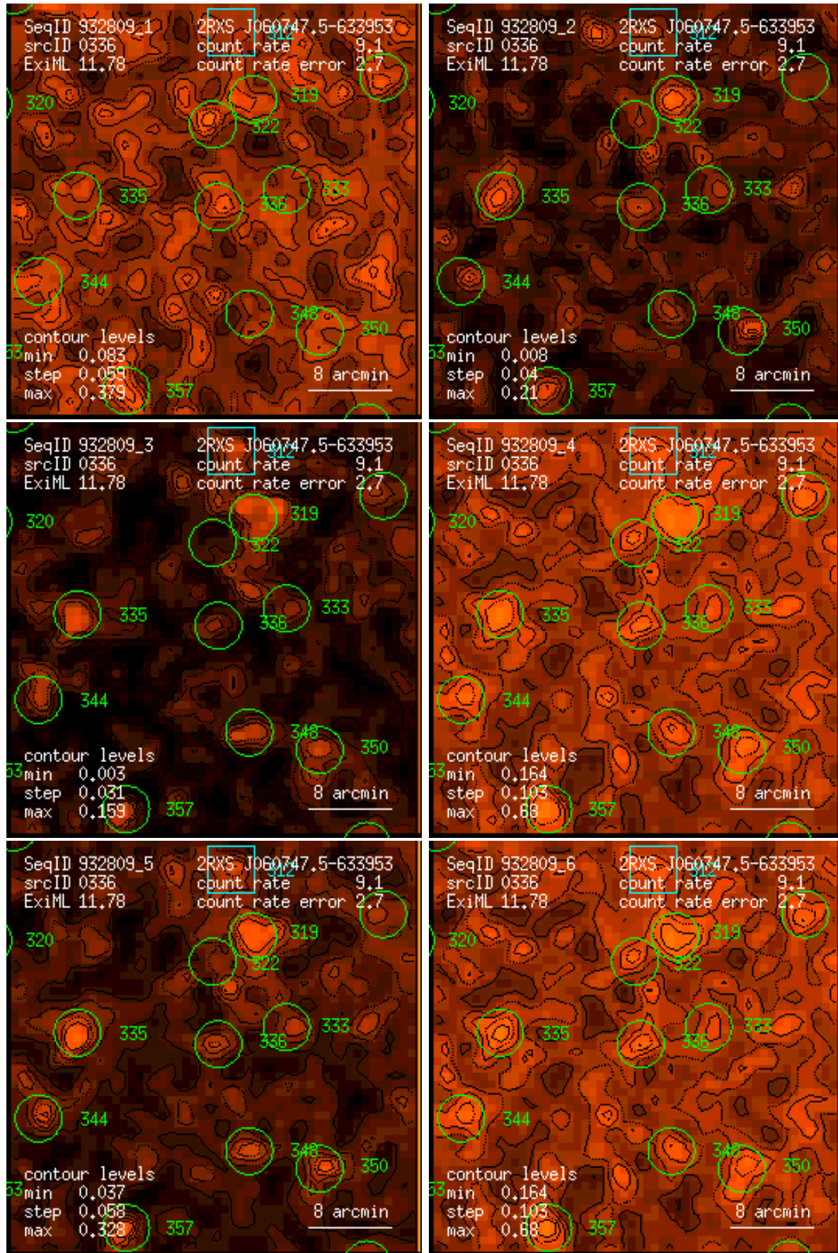
Figure 336: RASS 932809: detection 0336: band rate images, Gaussian filter: (1) PSPC channels 11 – 41, (2) 52 – 90, (3) 91 – 201, (4) 11 – 235, (5) 52 – 201, (6) 11 – 201. Broad band rates in counts/ks. Band rate contour levels in counts/ks/arcmin 2 .
