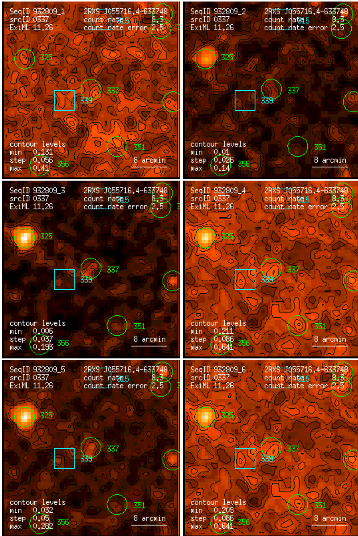
Figure 337: RASS 932809: detection 0337: band rate images, Gaussian filter: (1) PSPC channels 11 – 41, (2) 52 – 90, (3) 91 – 201, (4) 11 – 235, (5) 52 – 201, (6) 11 – 201. Broad band rates in counts/ks. Band rate contour levels in counts/ks/arcmin 2 .
