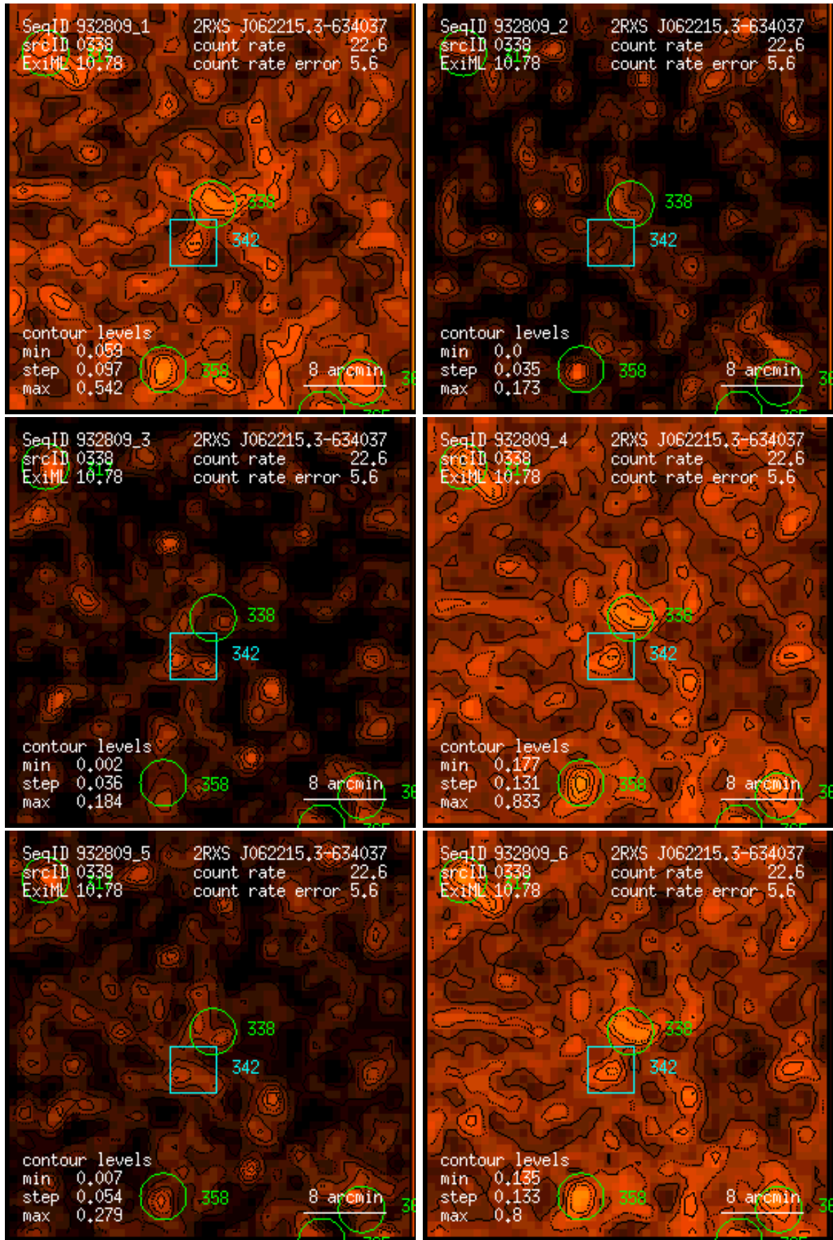
Figure 338: RASS 932809: detection 0338: band rate images, Gaussian filter: (1) PSPC channels 11 – 41, (2) 52 – 90, (3) 91 – 201, (4) 11 – 235, (5) 52 – 201, (6) 11 – 201. Broad band rates in counts/ks. Band rate contour levels in counts/ks/arcmin 2 .
