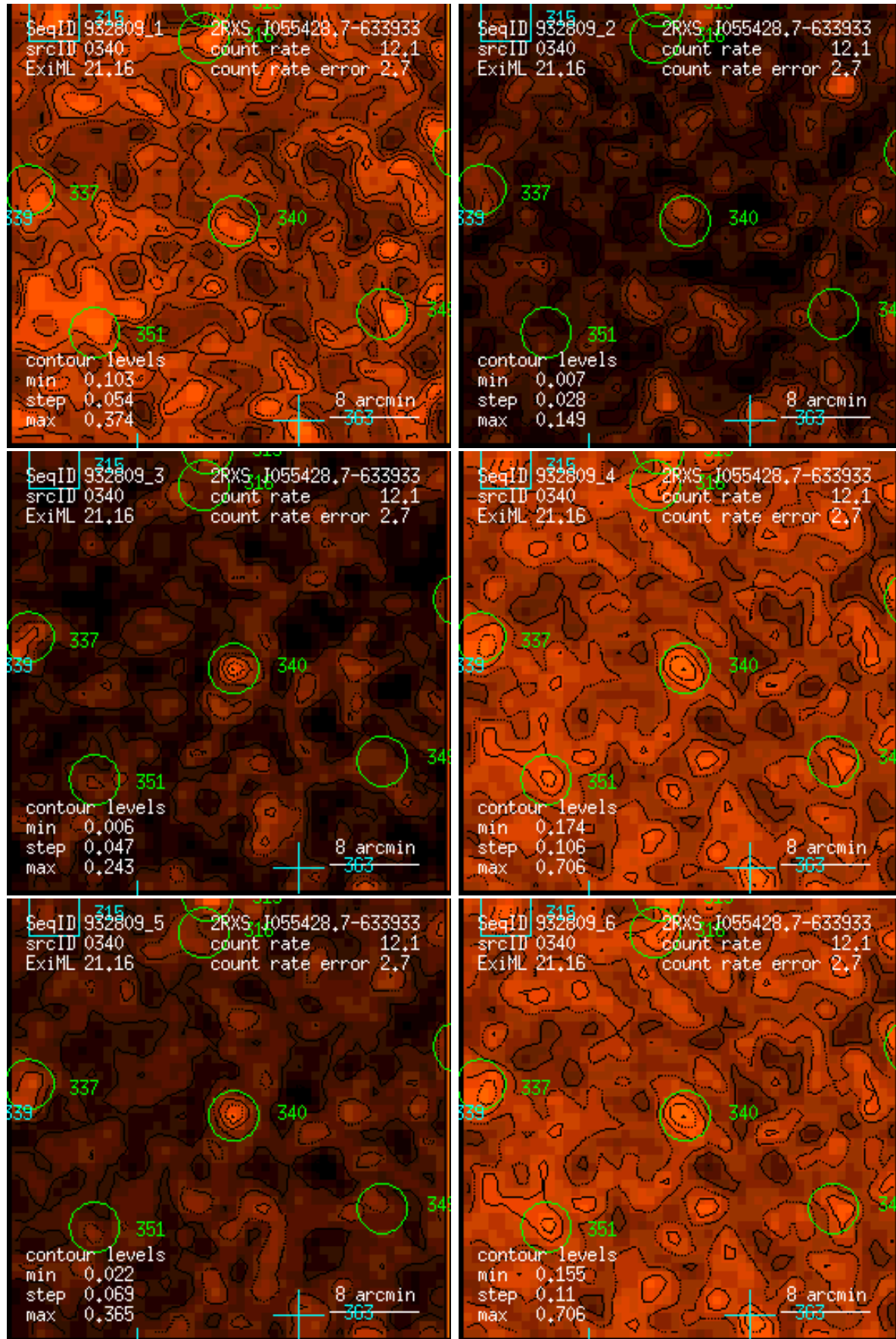
Figure 340: RASS 932809: detection 0340: band rate images, Gaussian filter: (1) PSPC channels 11 – 41, (2) 52 – 90, (3) 91 – 201, (4) 11 – 235, (5) 52 – 201, (6) 11 – 201. Broad band rates in counts/ks. Band rate contour levels in counts/ks/arcmin 2 .
