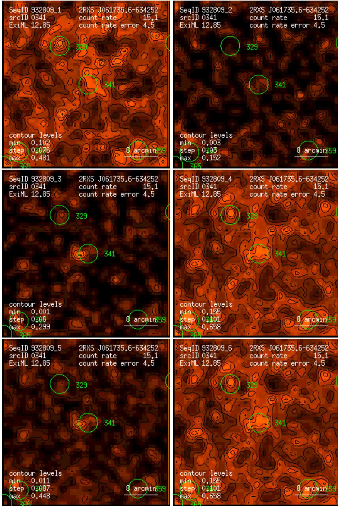
Figure 341: RASS 932809: detection 0341: band rate images, Gaussian filter: (1) PSPC channels 11 – 41, (2) 52 – 90, (3) 91 – 201, (4) 11 – 235, (5) 52 – 201, (6) 11 – 201. Broad band rates in counts/ks. Band rate contour levels in counts/ks/arcmin 2 .
