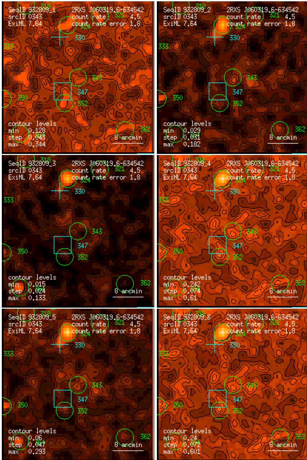
Figure 343: RASS 932809: detection 0343: band rate images, Gaussian filter: (1) PSPC channels 11 – 41, (2) 52 – 90, (3) 91 – 201, (4) 11 – 235, (5) 52 – 201, (6) 11 – 201. Broad band rates in counts/ks. Band rate contour levels in counts/ks/arcmin 2 .
