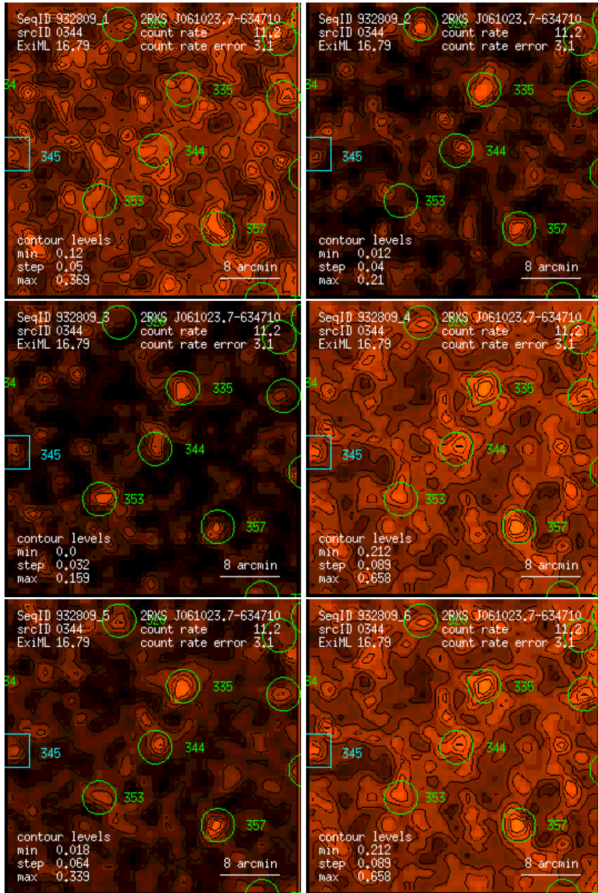
Figure 344: RASS 932809: detection 0344: band rate images, Gaussian filter: (1) PSPC channels 11 – 41, (2) 52 – 90, (3) 91 – 201, (4) 11 – 235, (5) 52 – 201, (6) 11 – 201. Broad band rates in counts/ks. Band rate contour levels in counts/ks/arcmin 2 .
