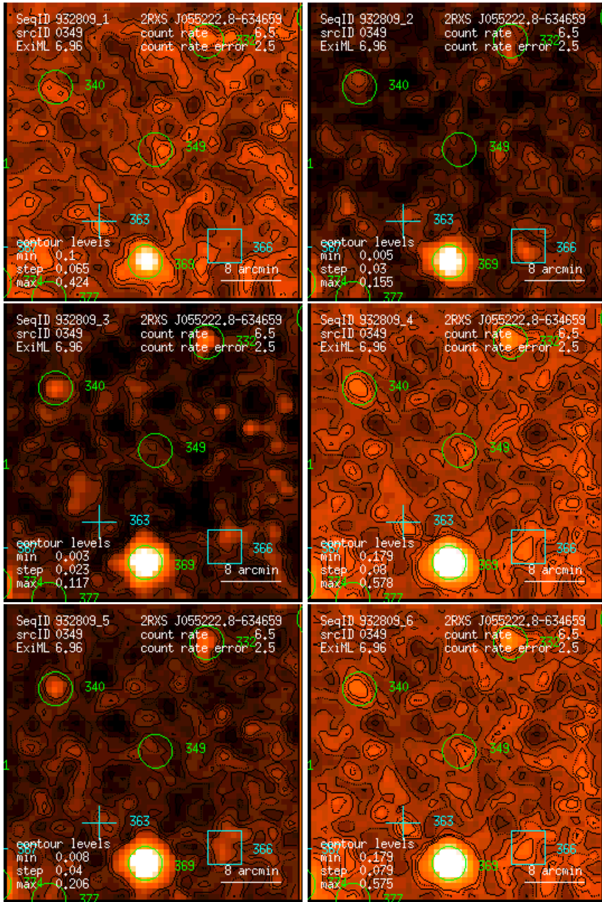
Figure 349: RASS 932809: detection 0349: band rate images, Gaussian filter: (1) PSPC channels 11 – 41, (2) 52 – 90, (3) 91 – 201, (4) 11 – 235, (5) 52 – 201, (6) 11 – 201. Broad band rates in counts/ks. Band rate contour levels in counts/ks/arcmin 2 .
