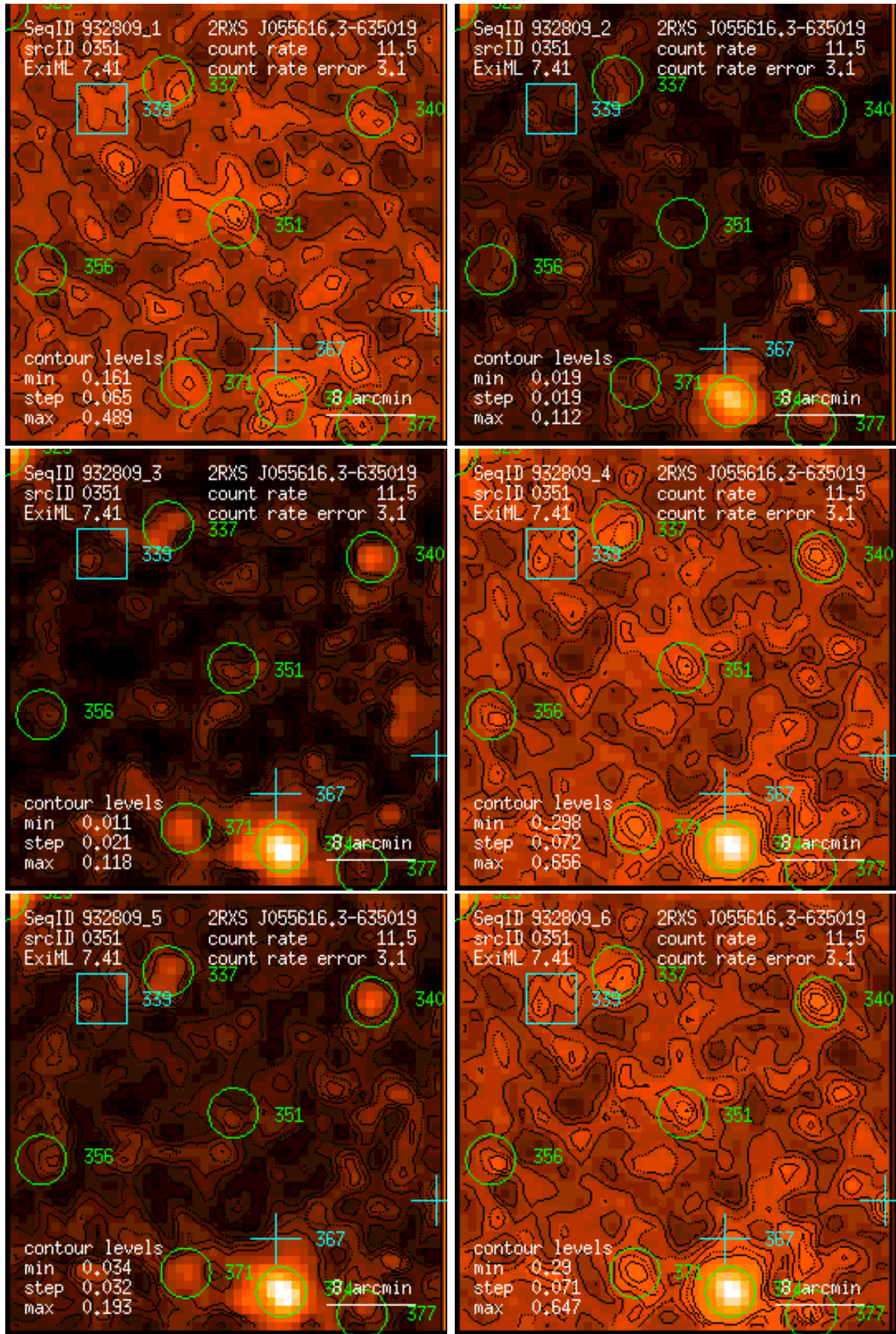
Figure 351: RASS 932809: detection 0351: band rate images, Gaussian filter: (1) PSPC channels 11 – 41, (2) 52 – 90, (3) 91 – 201, (4) 11 – 235, (5) 52 – 201, (6) 11 – 201. Broad band rates in counts/ks. Band rate contour levels in counts/ks/arcmin 2 .
