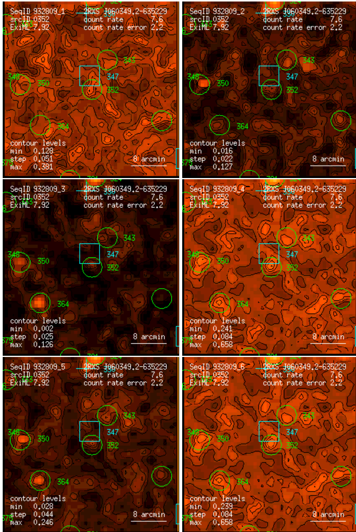
Figure 352: RASS 932809: detection 0352: band rate images, Gaussian filter: (1) PSPC channels 11 – 41, (2) 52 – 90, (3) 91 – 201, (4) 11 – 235, (5) 52 – 201, (6) 11 – 201. Broad band rates in counts/ks. Band rate contour levels in counts/ks/arcmin 2 .
