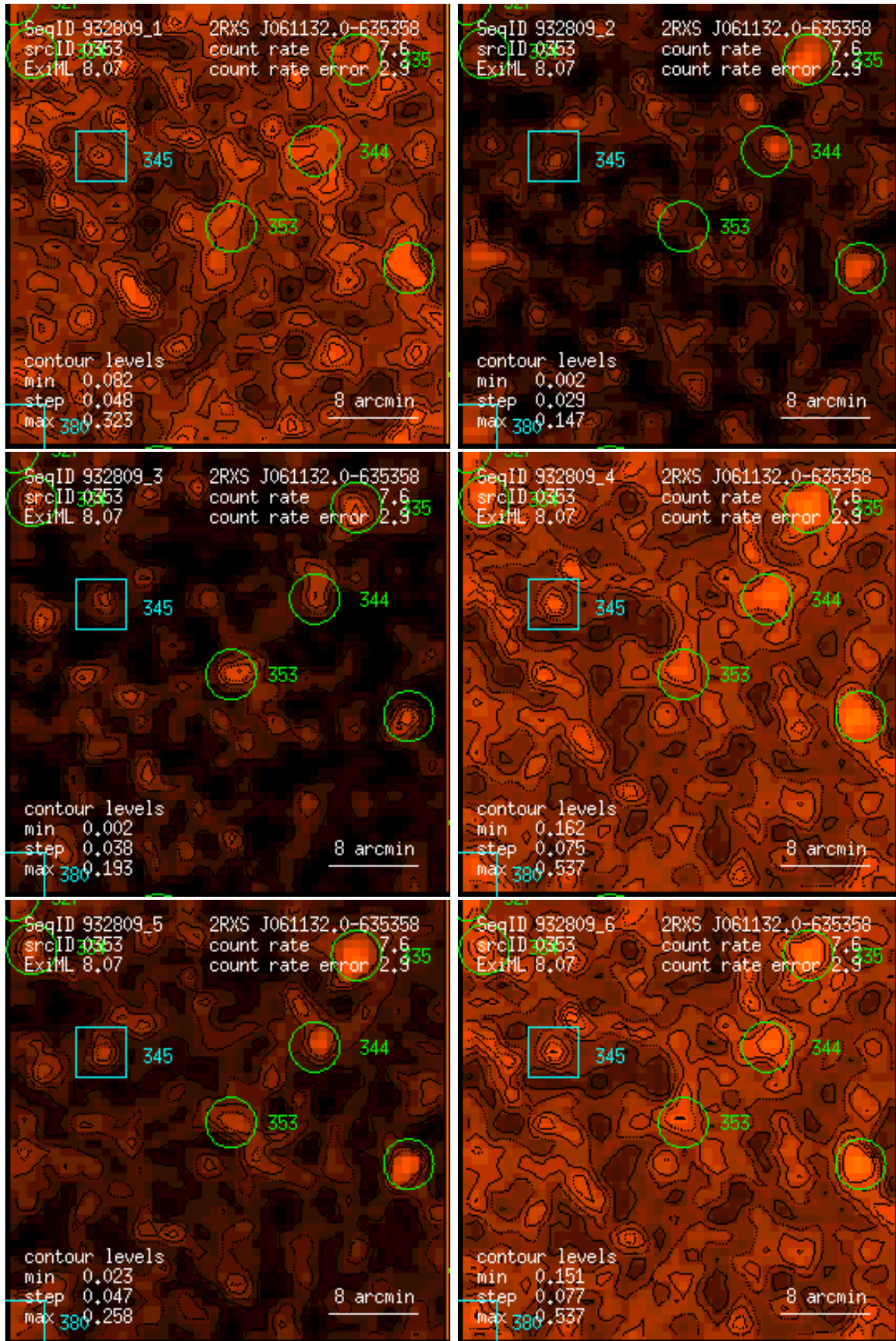
Figure 353: RASS 932809: detection 0353: band rate images, Gaussian filter: (1) PSPC channels 11 – 41, (2) 52 – 90, (3) 91 – 201, (4) 11 – 235, (5) 52 – 201, (6) 11 – 201. Broad band rates in counts/ks. Band rate contour levels in counts/ks/arcmin 2 .
