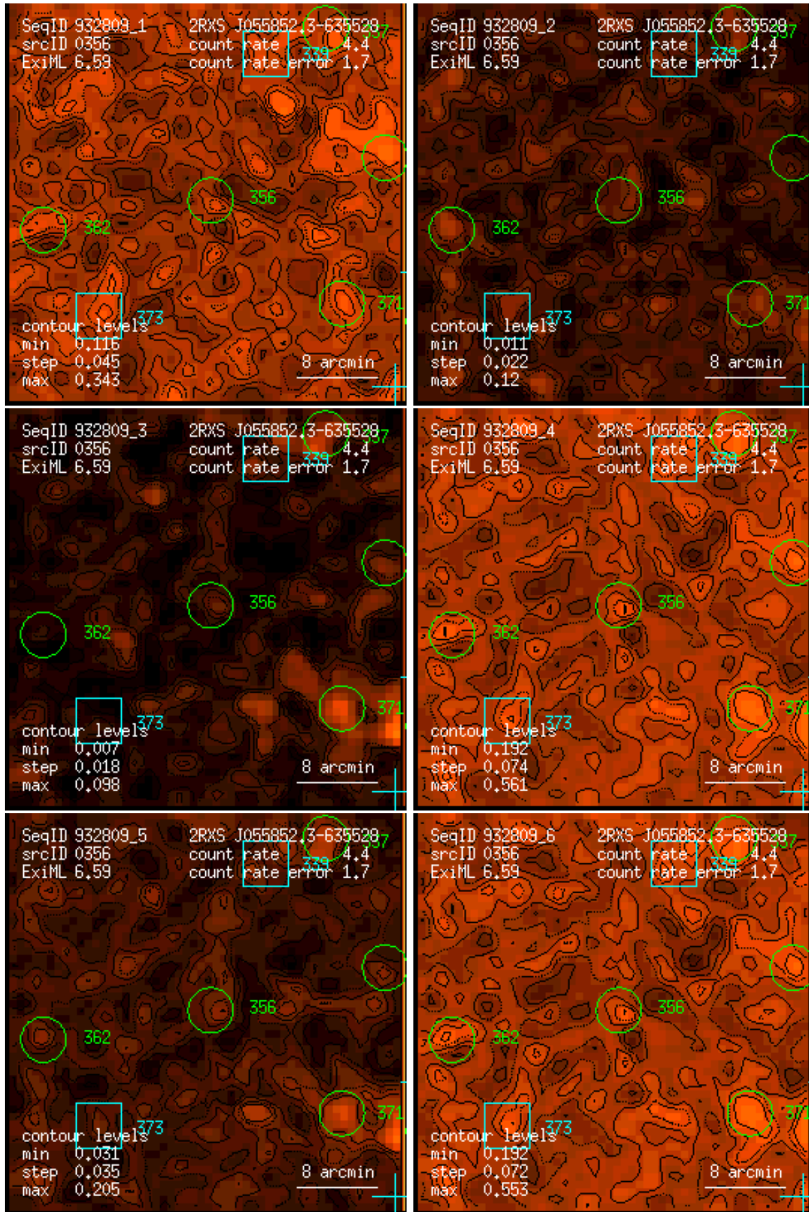
Figure 356: RASS 932809: detection 0356: band rate images, Gaussian filter: (1) PSPC channels 11 – 41, (2) 52 – 90, (3) 91 – 201, (4) 11 – 235, (5) 52 – 201, (6) 11 – 201. Broad band rates in counts/ks. Band rate contour levels in counts/ks/arcmin 2 .
