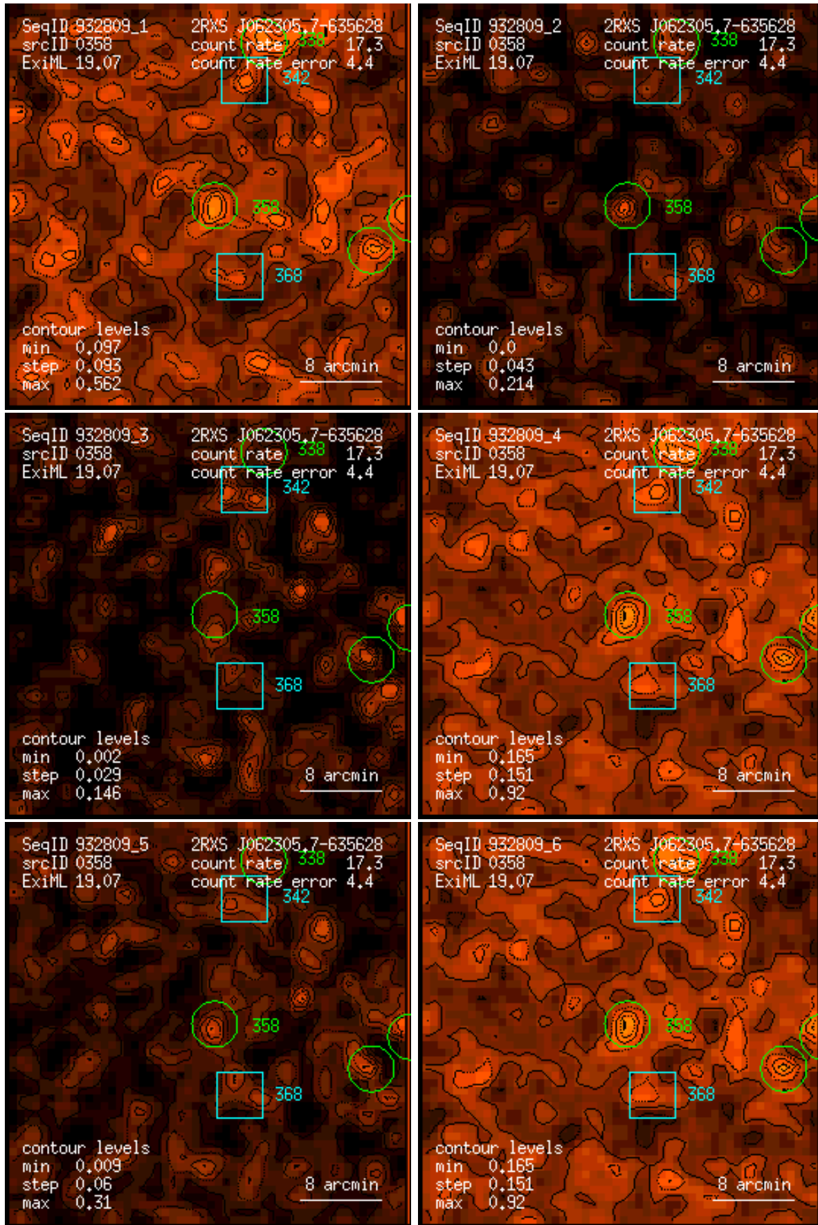
Figure 358: RASS 932809: detection 0358: band rate images, Gaussian filter: (1) PSPC channels 11 – 41, (2) 52 – 90, (3) 91 – 201, (4) 11 – 235, (5) 52 – 201, (6) 11 – 201. Broad band rates in counts/ks. Band rate contour levels in counts/ks/arcmin 2 .
