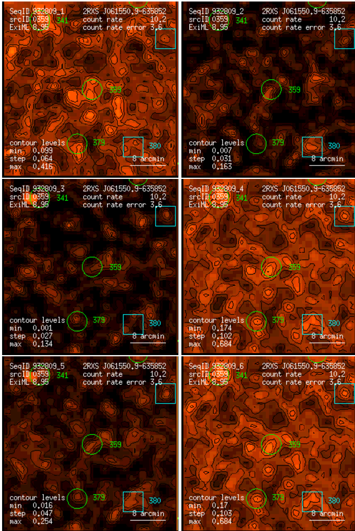
Figure 359: RASS 932809: detection 0359: band rate images, Gaussian filter: (1) PSPC channels 11 – 41, (2) 52 – 90, (3) 91 – 201, (4) 11 – 235, (5) 52 – 201, (6) 11 – 201. Broad band rates in counts/ks. Band rate contour levels in counts/ks/arcmin 2 .
