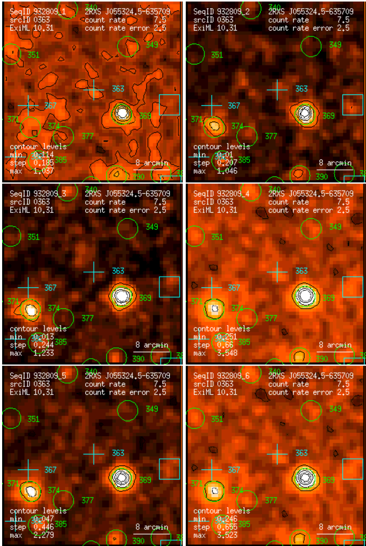
Figure 363: RASS 932809: detection 0363: band rate images, Gaussian filter: (1) PSPC channels 11 – 41, (2) 52 – 90, (3) 91 – 201, (4) 11 – 235, (5) 52 – 201, (6) 11 – 201. Broad band rates in counts/ks. Band rate contour levels in counts/ks/arcmin 2 .
