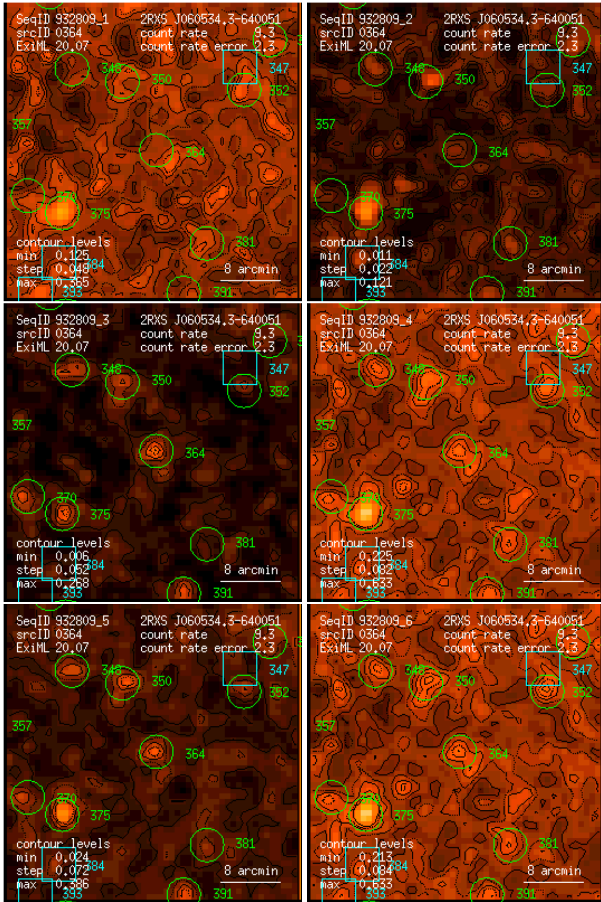
Figure 364: RASS 932809: detection 0364: band rate images, Gaussian filter: (1) PSPC channels 11 – 41, (2) 52 – 90, (3) 91 – 201, (4) 11 – 235, (5) 52 – 201, (6) 11 – 201. Broad band rates in counts/ks. Band rate contour levels in counts/ks/arcmin 2 .
