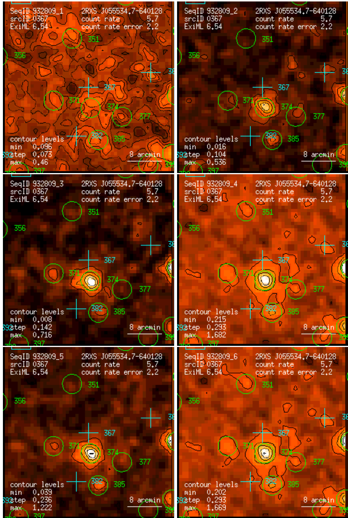
Figure 367: RASS 932809: detection 0367: band rate images, Gaussian filter: (1) PSPC channels 11 – 41, (2) 52 – 90, (3) 91 – 201, (4) 11 – 235, (5) 52 – 201, (6) 11 – 201. Broad band rates in counts/ks. Band rate contour levels in counts/ks/arcmin 2 .
