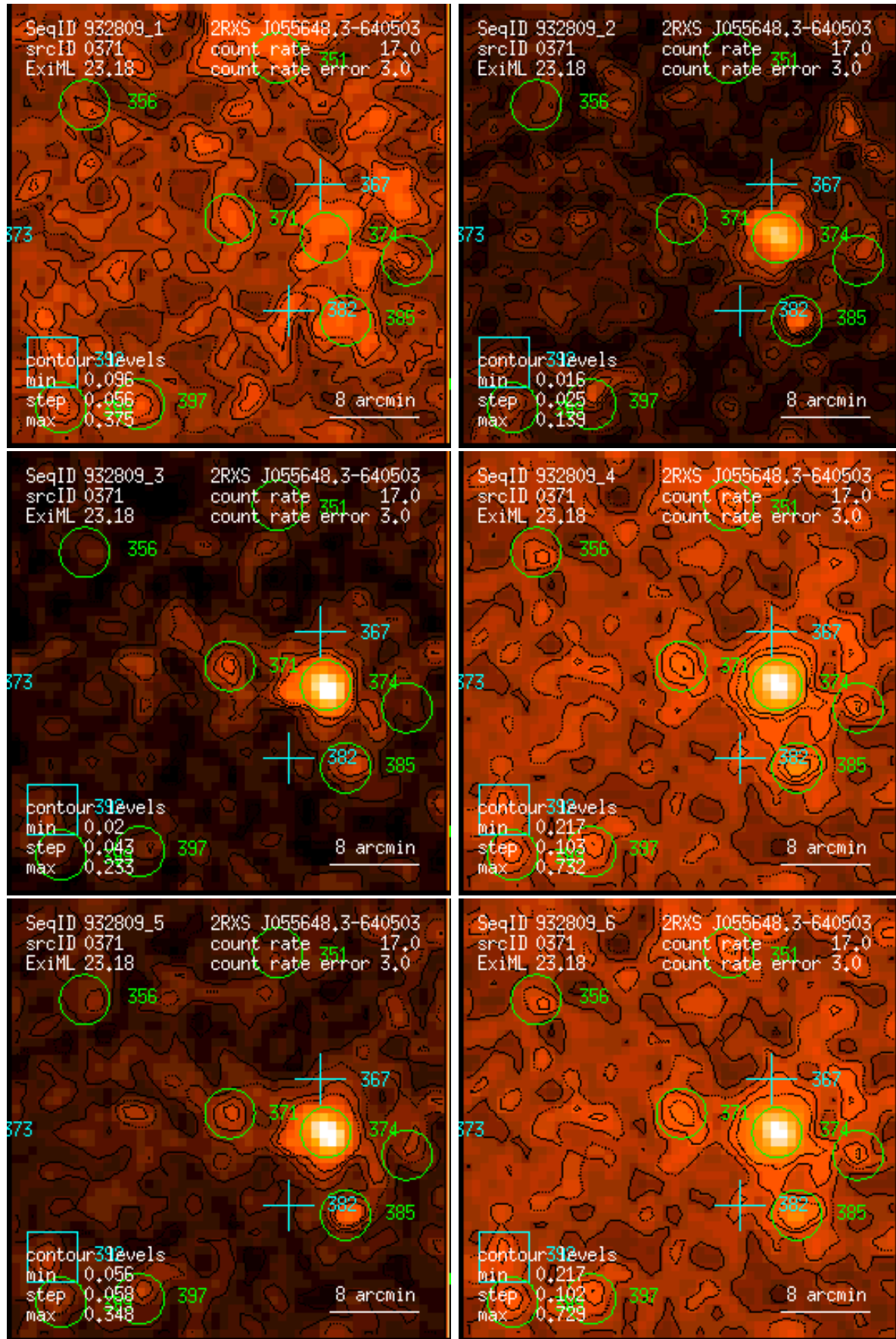
Figure 371: RASS 932809: detection 0371: band rate images, Gaussian filter: (1) PSPC channels 11 – 41, (2) 52 – 90, (3) 91 – 201, (4) 11 – 235, (5) 52 – 201, (6) 11 – 201. Broad band rates in counts/ks. Band rate contour levels in counts/ks/arcmin 2 .
