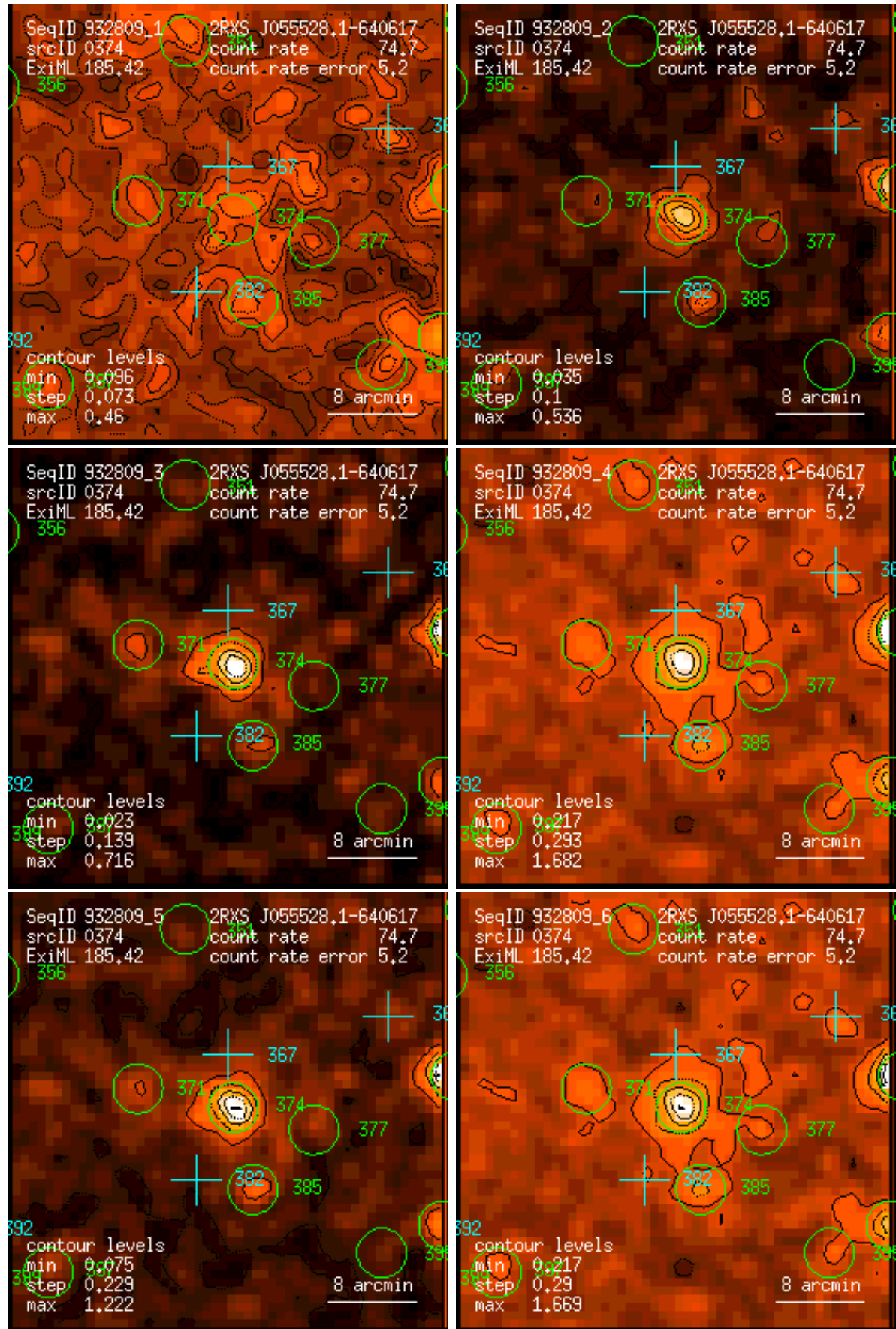
Figure 374: RASS 932809: detection 0374: band rate images, Gaussian filter: (1) PSPC channels 11 – 41, (2) 52 – 90, (3) 91 – 201, (4) 11 – 235, (5) 52 – 201, (6) 11 – 201. Broad band rates in counts/ks. Band rate contour levels in counts/ks/arcmin 2 .
