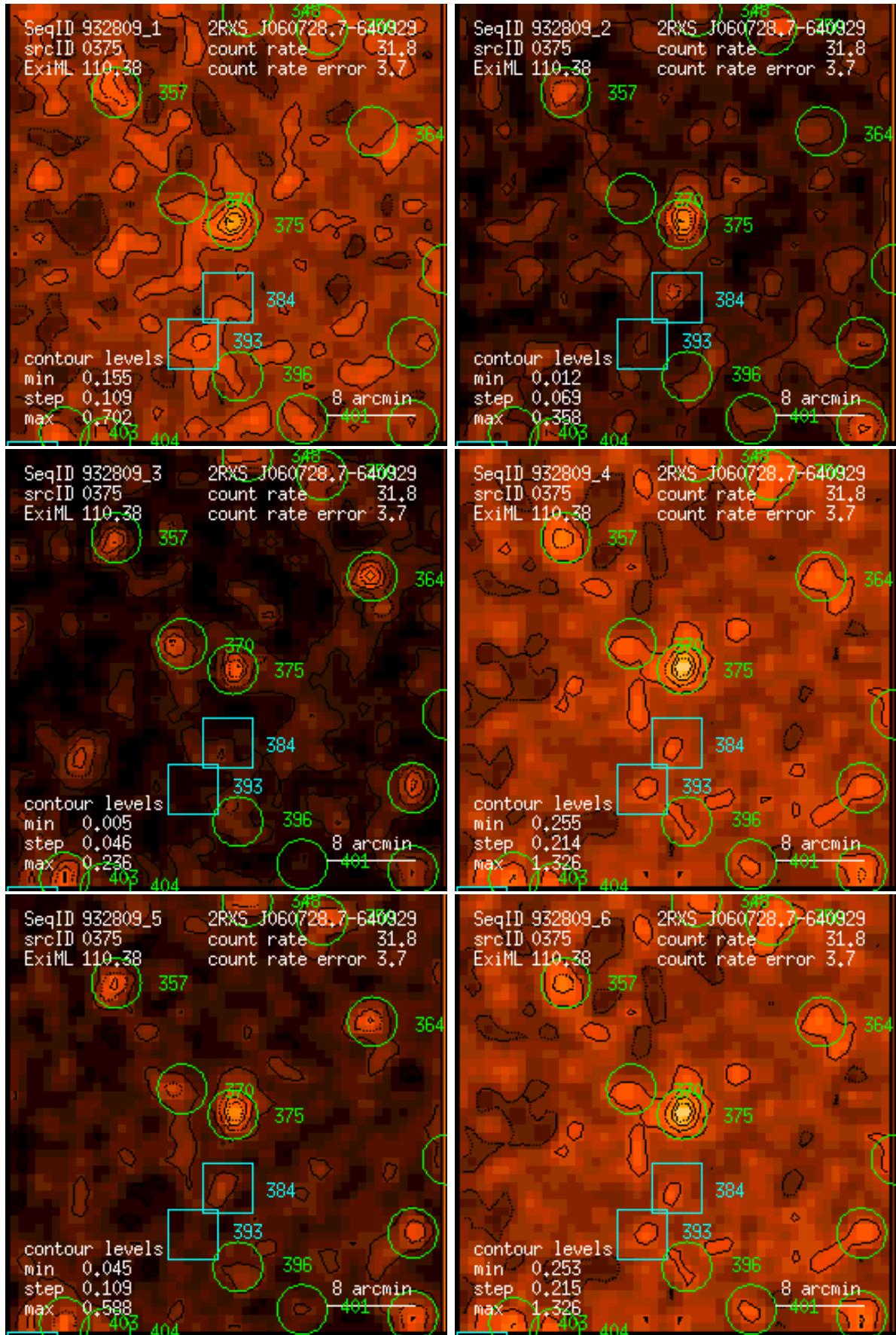
Figure 375: RASS 932809: detection 0375: band rate images, Gaussian filter: (1) PSPC channels 11 – 41, (2) 52 – 90, (3) 91 – 201, (4) 11 – 235, (5) 52 – 201, (6) 11 – 201. Broad band rates in counts/ks. Band rate contour levels in counts/ks/arcmin 2 .
