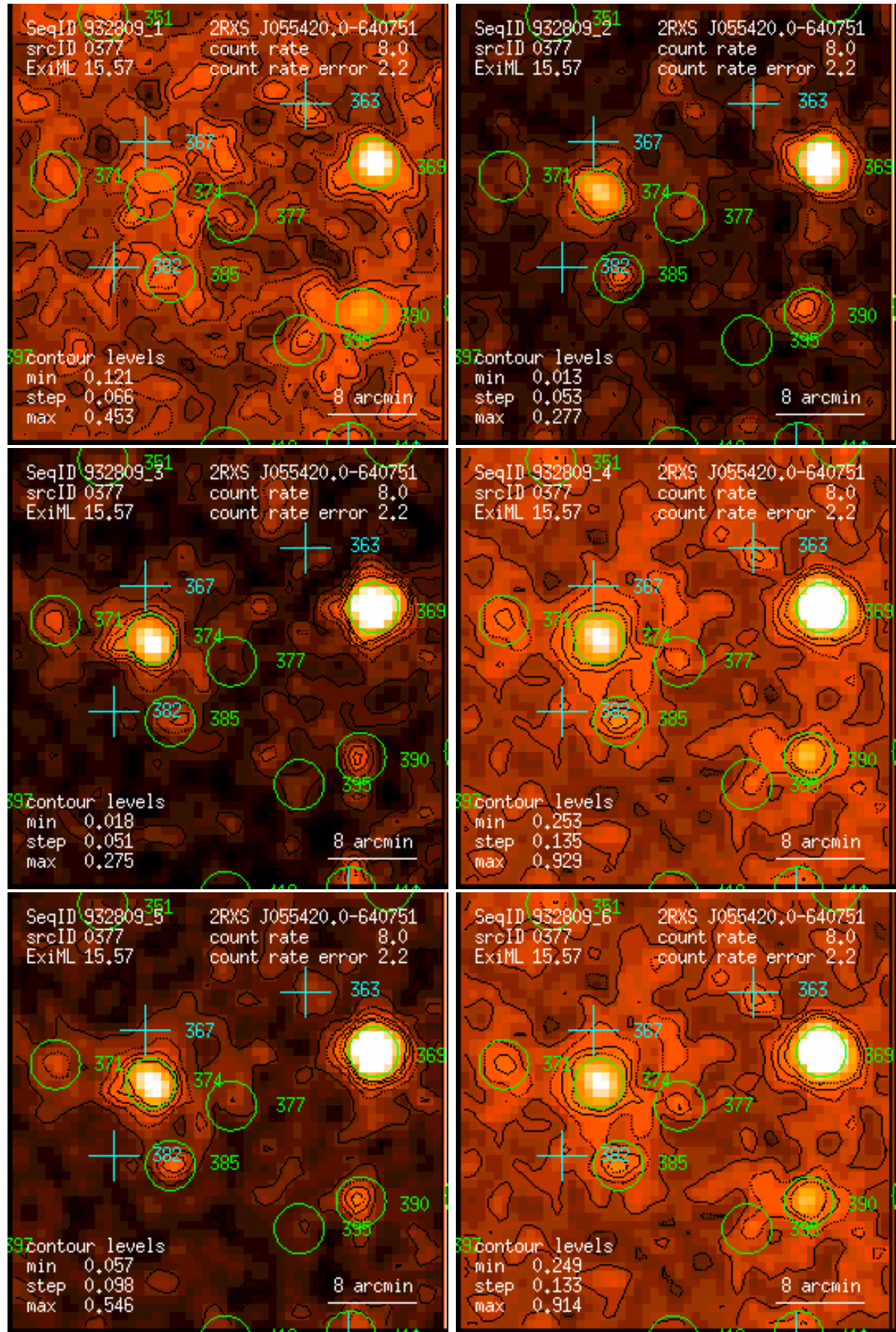
Figure 377: RASS 932809: detection 0377: band rate images, Gaussian filter: (1) PSPC channels 11 – 41, (2) 52 – 90, (3) 91 – 201, (4) 11 – 235, (5) 52 – 201, (6) 11 – 201. Broad band rates in counts/ks. Band rate contour levels in counts/ks/arcmin 2 .
