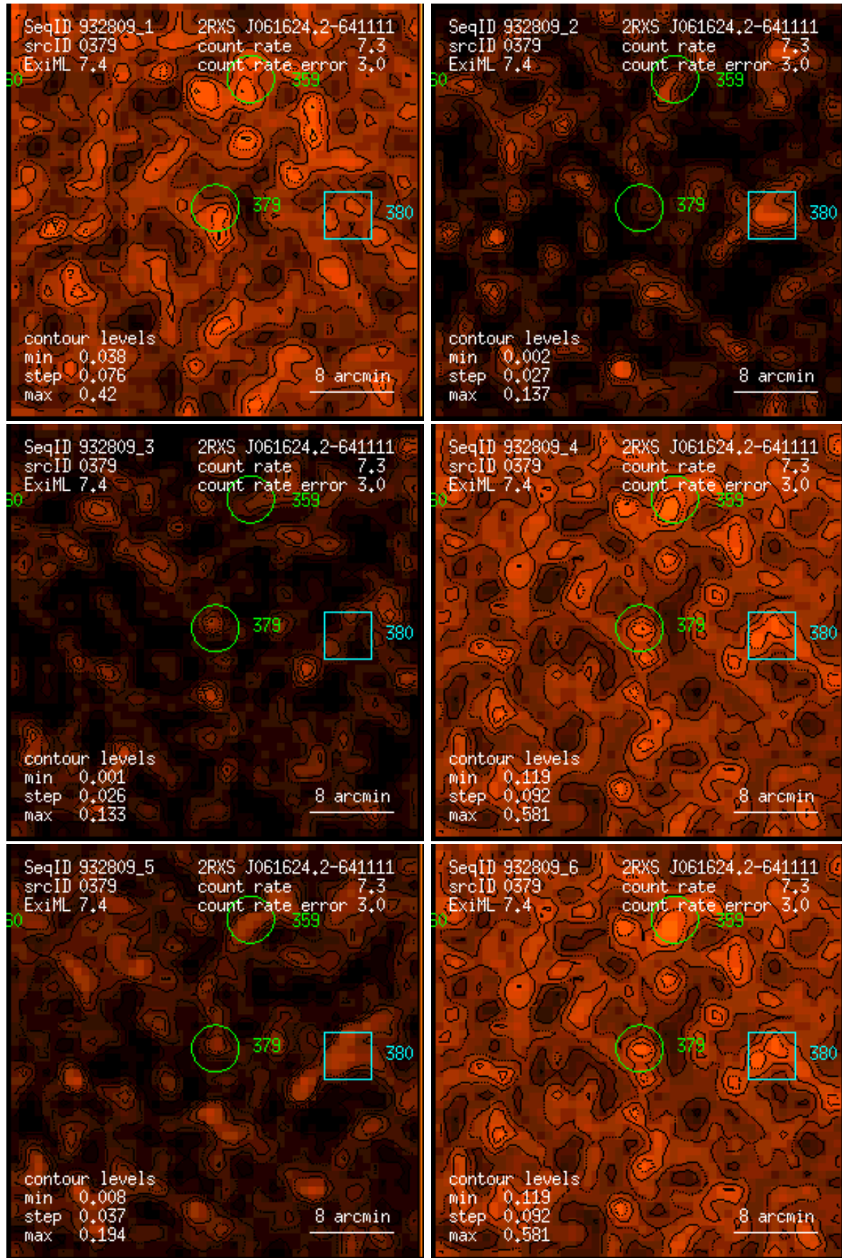
Figure 379: RASS 932809: detection 0379: band rate images, Gaussian filter: (1) PSPC channels 11 – 41, (2) 52 – 90, (3) 91 – 201, (4) 11 – 235, (5) 52 – 201, (6) 11 – 201. Broad band rates in counts/ks. Band rate contour levels in counts/ks/arcmin 2 .
