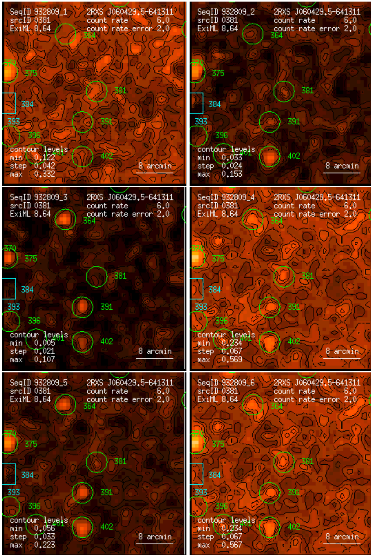
Figure 381: RASS 932809: detection 0381: band rate images, Gaussian filter: (1) PSPC channels 11 – 41, (2) 52 – 90, (3) 91 – 201, (4) 11 – 235, (5) 52 – 201, (6) 11 – 201. Broad band rates in counts/ks. Band rate contour levels in counts/ks/arcmin 2 .
