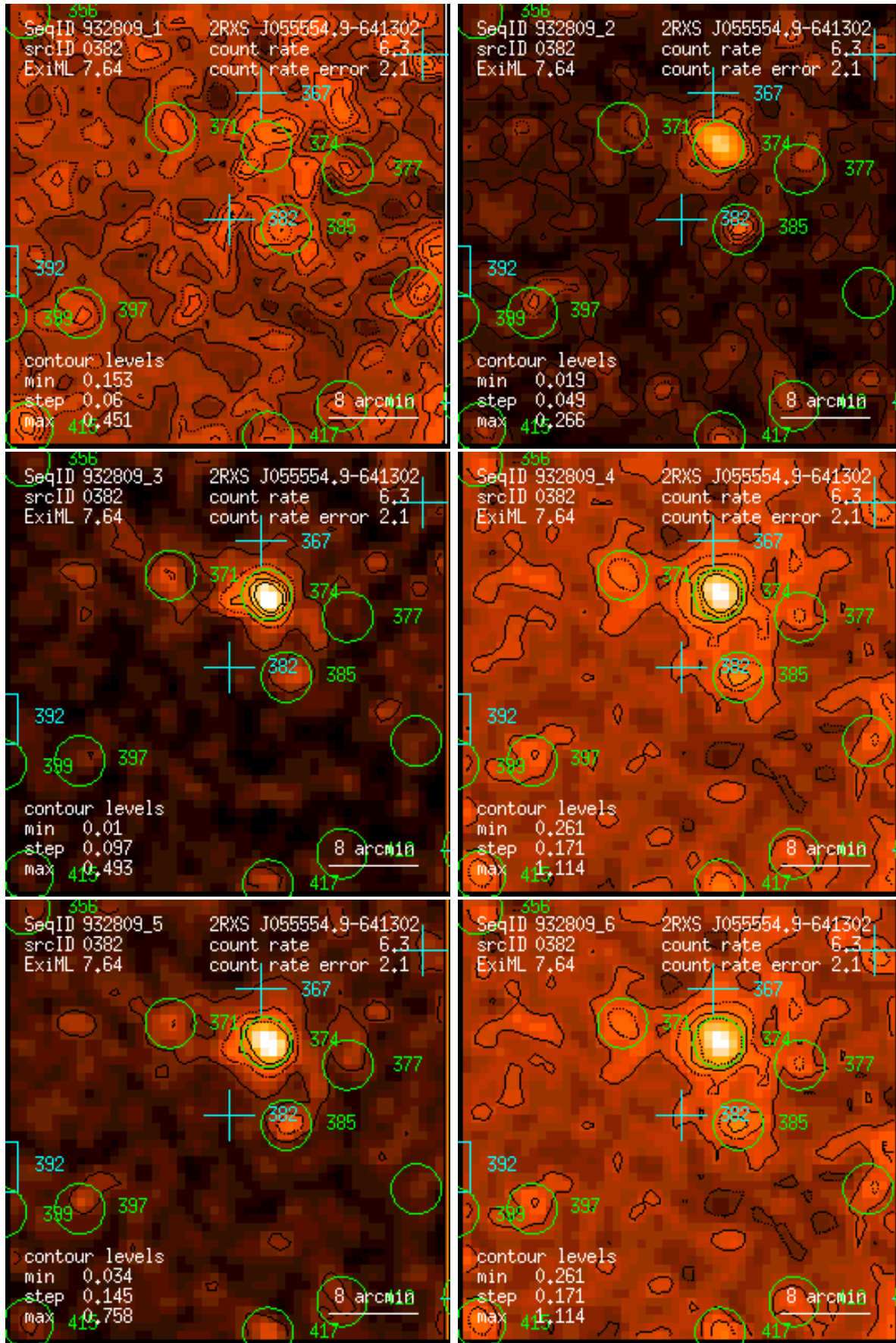
Figure 382: RASS 932809: detection 0382: band rate images, Gaussian filter: (1) PSPC channels 11 – 41, (2) 52 – 90, (3) 91 – 201, (4) 11 – 235, (5) 52 – 201, (6) 11 – 201. Broad band rates in counts/ks. Band rate contour levels in counts/ks/arcmin 2 .
