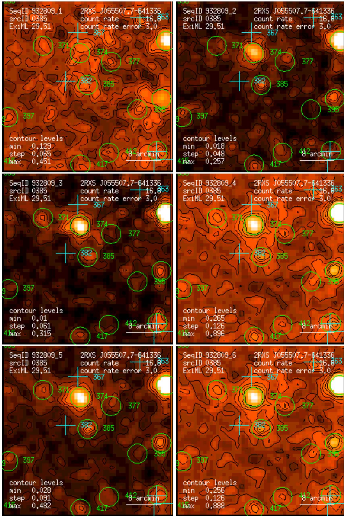
Figure 385: RASS 932809: detection 0385: band rate images, Gaussian filter: (1) PSPC channels 11 – 41, (2) 52 – 90, (3) 91 – 201, (4) 11 – 235, (5) 52 – 201, (6) 11 – 201. Broad band rates in counts/ks. Band rate contour levels in counts/ks/arcmin 2 .
