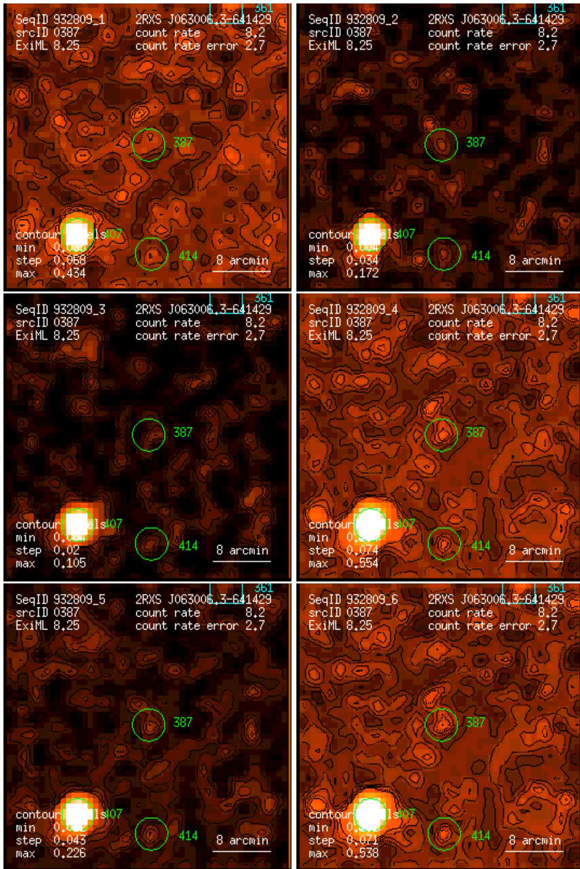
Figure 387: RASS 932809: detection 0387: band rate images, Gaussian filter: (1) PSPC channels 11 – 41, (2) 52 – 90, (3) 91 – 201, (4) 11 – 235, (5) 52 – 201, (6) 11 – 201. Broad band rates in counts/ks. Band rate contour levels in counts/ks/arcmin 2 .
